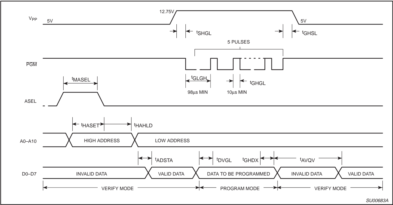
Figure 22. Program/Verify Cycle
