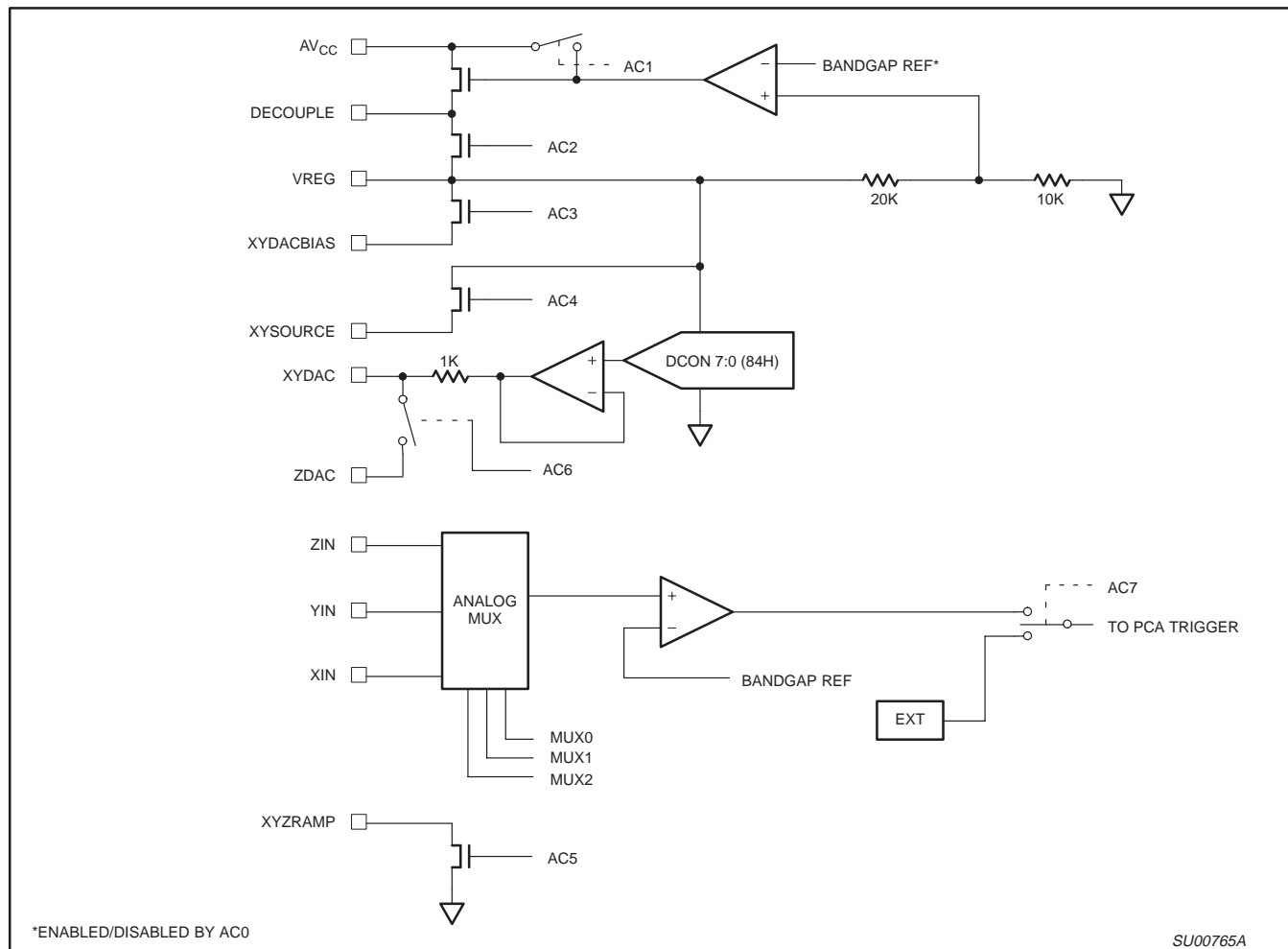
Figure 3. Analog Section
