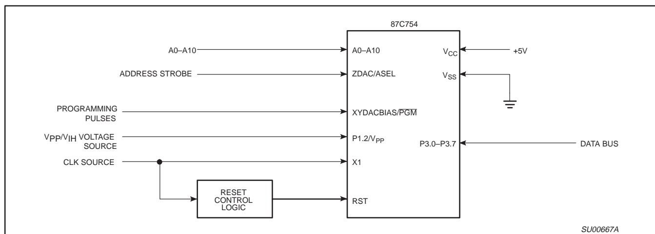
Figure 20. Programming Configuration
