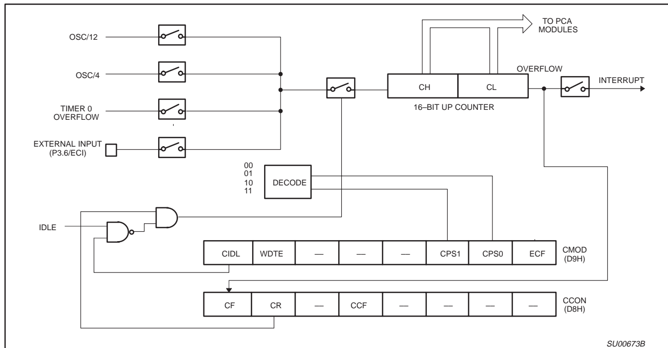
Figure 6. PCA Timer/Counter
