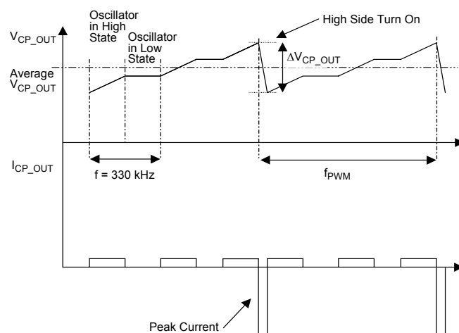
Figure 9. Simplified C CP_OUT Current and Voltage Waveforms
