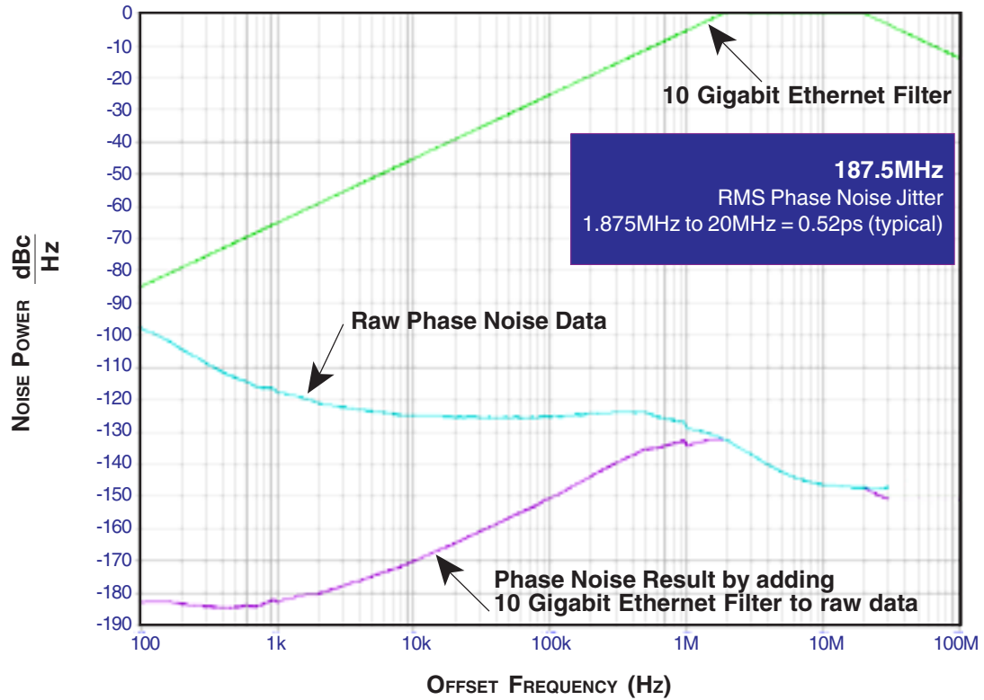
TYPICAL PHASE NOISE AT 187.5MHz
