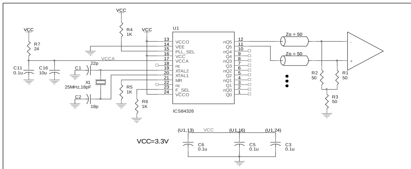
FIGURE 5A. ICS84326 SCHEMATIC EXAMPLE
