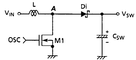
Figure 10 Switching regulator
