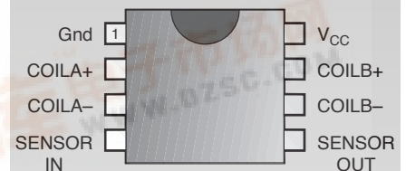
8L PDIP
