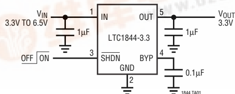
Fixed Voltage Low Noise, VLDO Linear Regulator
