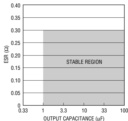
Figure 3. Stability
