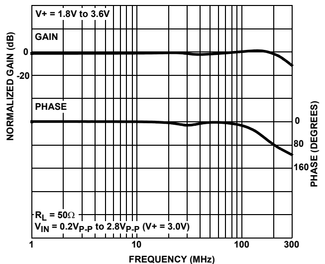
FIGURE 14. FREQUENCY RESPONSE
