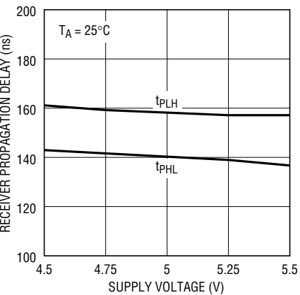
Receiver Propagation Delay vs Supply Voltage
