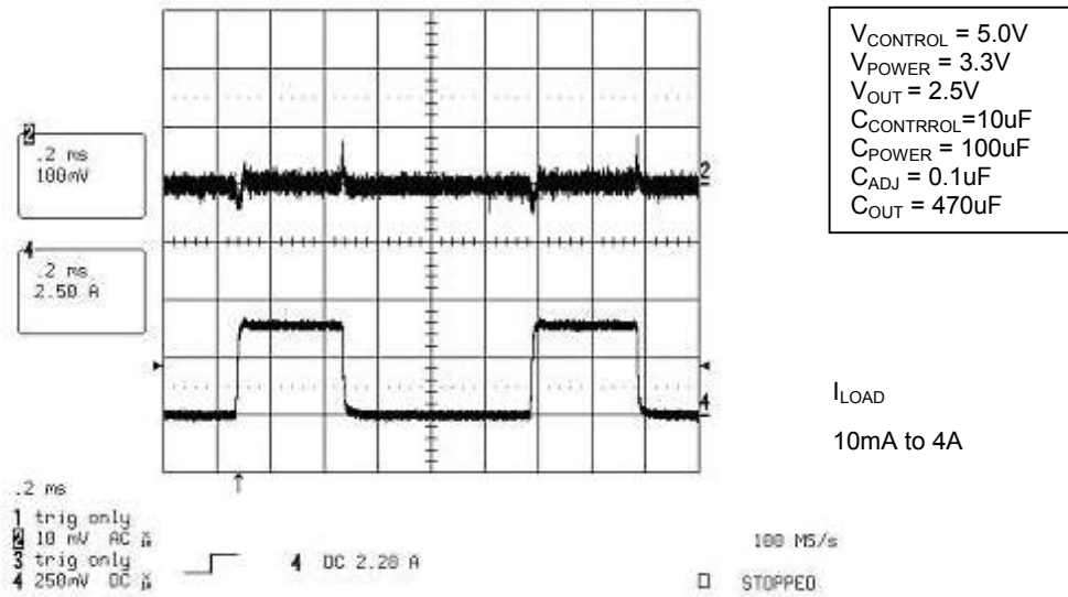
Transient Response
