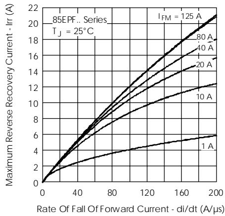
Fig.12-RecoveryCurrentCharacteristics, T_J = 25^\circ\text{C}
