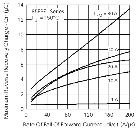
Fig.11-RecoveryChargeCharacteristics, T_J = 150^\circ\text{C}
