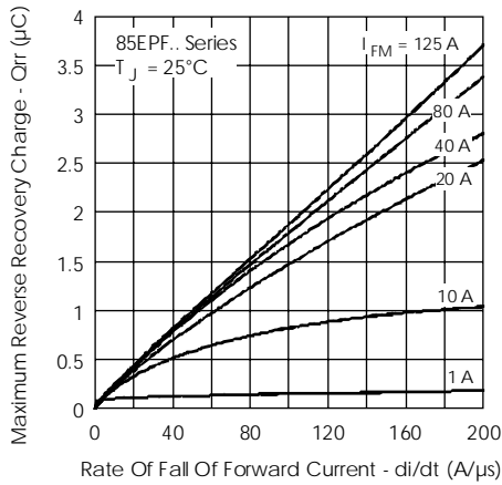
Fig.10-RecoveryChargeCharacteristics, T_J = 25^\circ\text{C}
