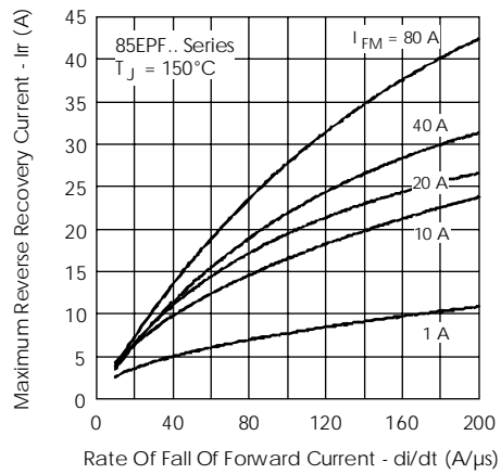
Fig.13-RecoveryCurrentCharacteristics, T_J = 150^\circ\text{C}
