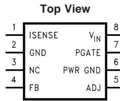
8 Lead Plastic MSOP-8 NS package Number MUA08A
