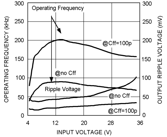
Feed-Forward Capacitor ( C_{\text{ff}} ) Effect ( V_{\text{OUT}} = 3.3\text{V} , L = 22\mu\text{H} , I_{\text{OUT}} = 500\text{mA} )
