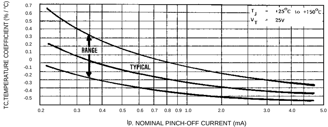
FIGURE 2 TEMPERATURE COEFFICIENT
