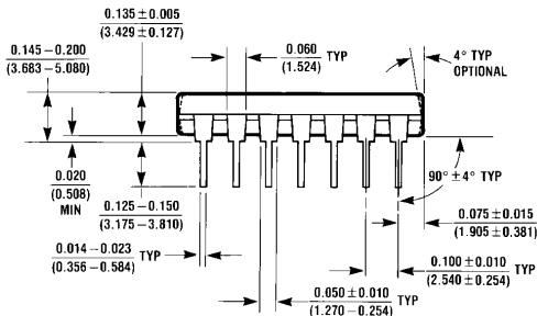
Molded Dual-In-Line Package (N) Order Number LM319AN or LM319N NS Package Number N14A
