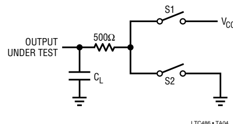
Figure 3. Driver Timing Test Load #2
