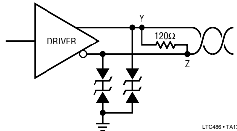
Figure 12. ESD Protection
