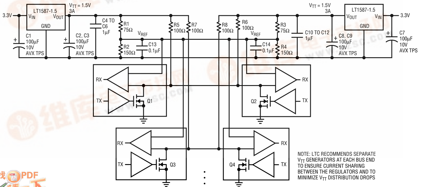
Intel Pentium Pro Processor GTL+ Supply
