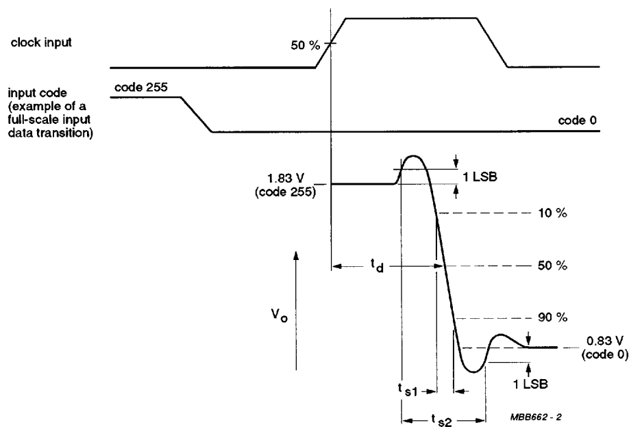
Fig.4 Switching timing.
