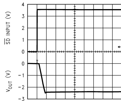
Start-up from Shutdown (no load)
