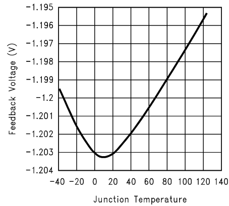
V_{\text{FB}} vs. Temperature
