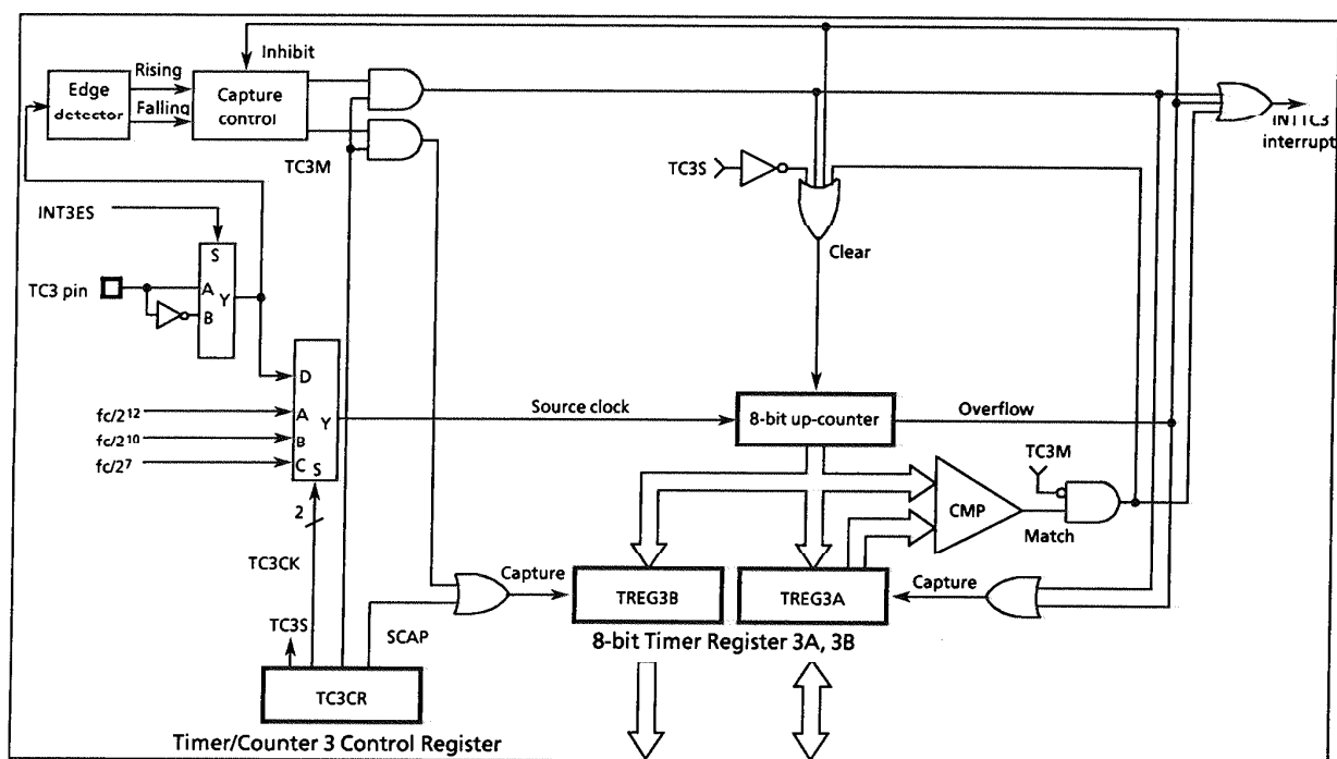
Figure 2-15. Timer/Counter 3
