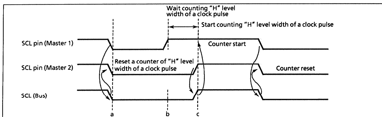
Figure 2-2/. Clock synchronization
