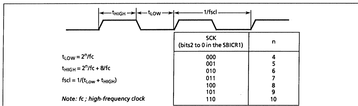
Figure 2-26. Clock source
