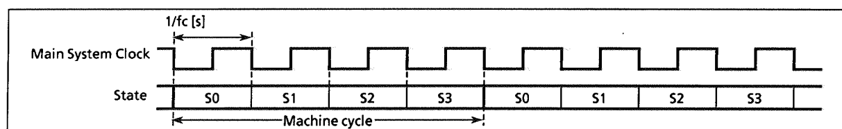
Figure 1-12. Machine cycle
