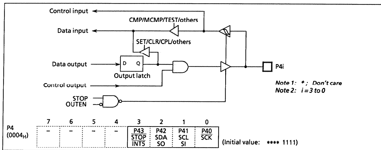
Figure 2-4. Port P4
