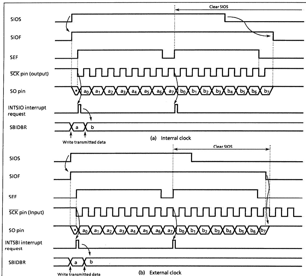
Figure 2-42. Transfer mode
