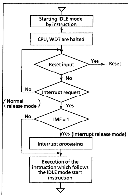
Figure 1-18. IDLE mode
