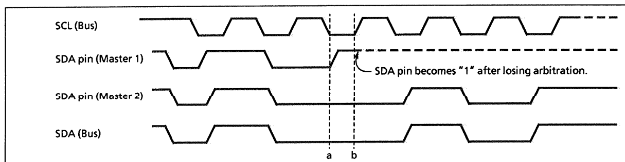
Figure 2-30. Arbitration lost
