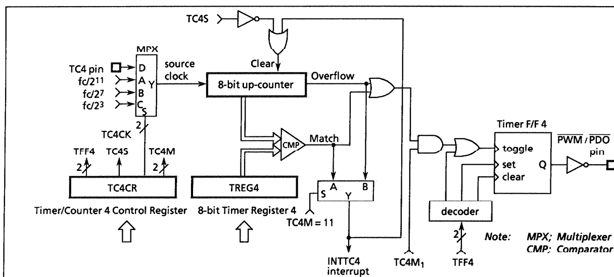
Figure 2-18. Timer/Counter 4
