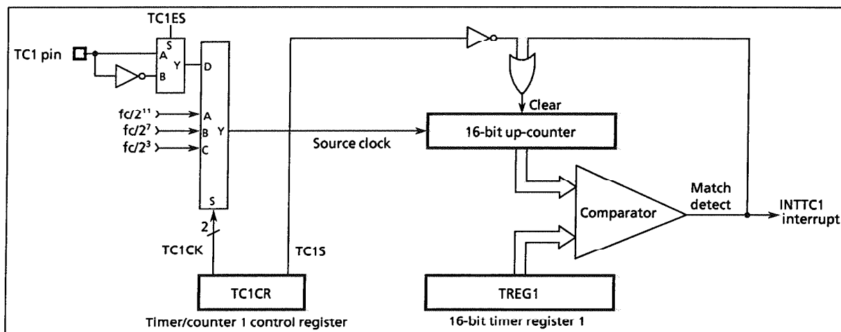
Figure 2-11. Timer/Counter 1
