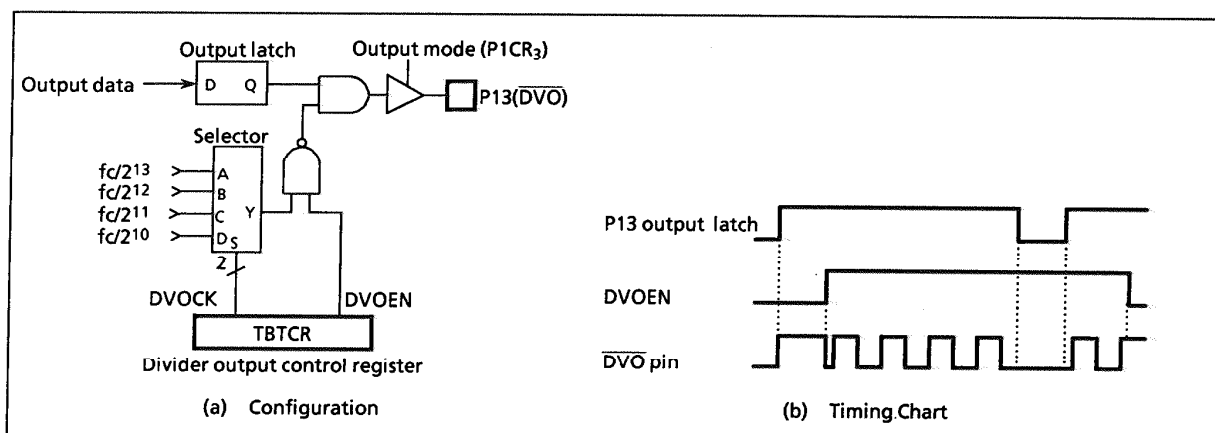
Figure 2-10. Divider output
