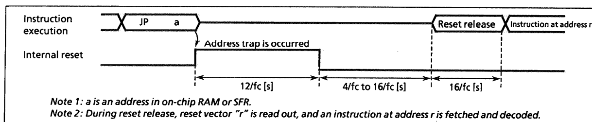
Figure 1-29. Address trap reset
