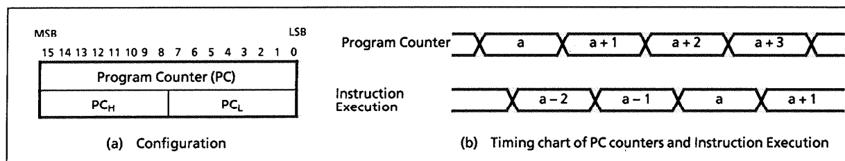
Figure 1-3. Program counter
