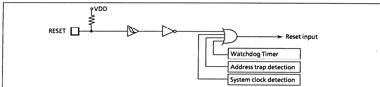
Figure 1-28. Reset circuit
