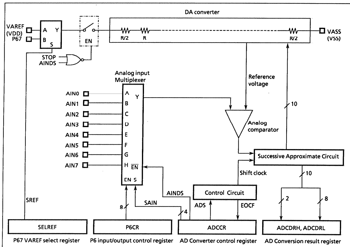
Figure 2-51. AD Converter
