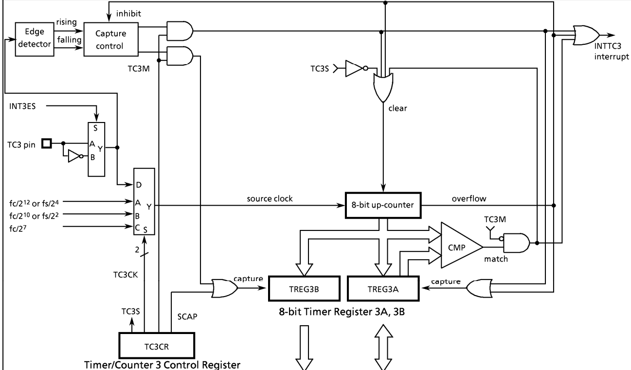
Figure 2-22. Timer/Counter 3
