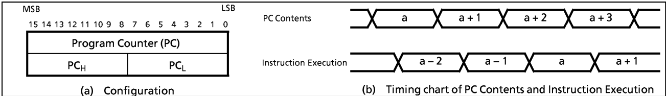
Figure 1-3. Program Counter
