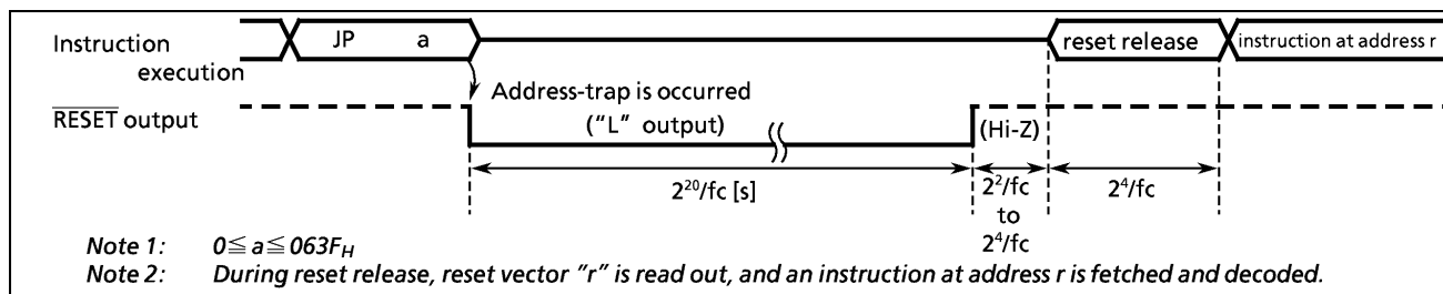
Figure 1-31. Address-Trap-Reset
