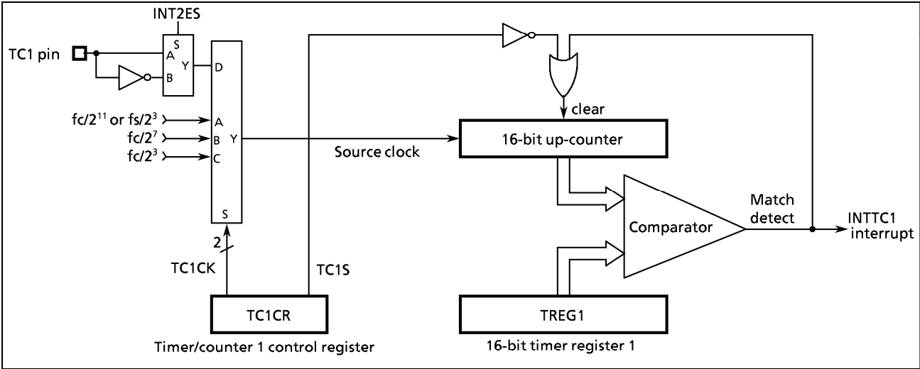
Figure 2-16. Timer/Couter 1
