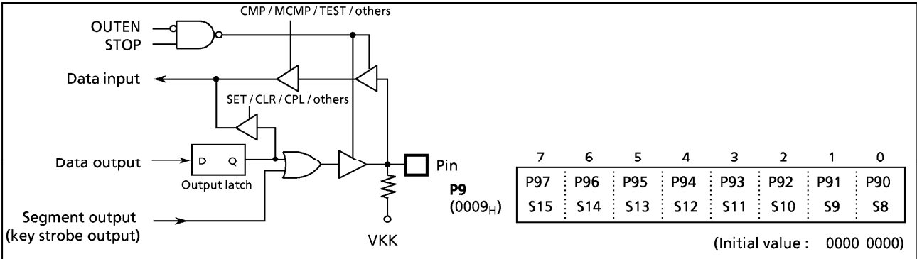
Figure 2-11. Port P9
