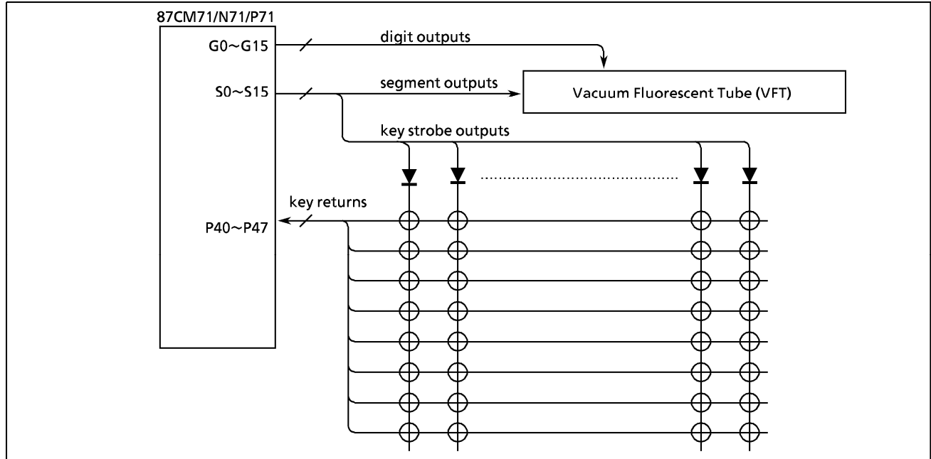
Figure 2-48. Key Matrix Example
