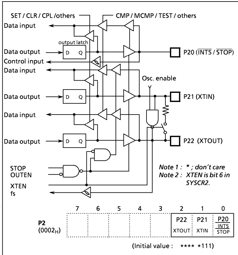
Figure 2-5. Port P2
