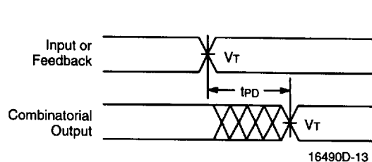
Combinatorial Output
