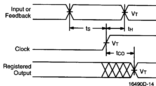
Registered Output
