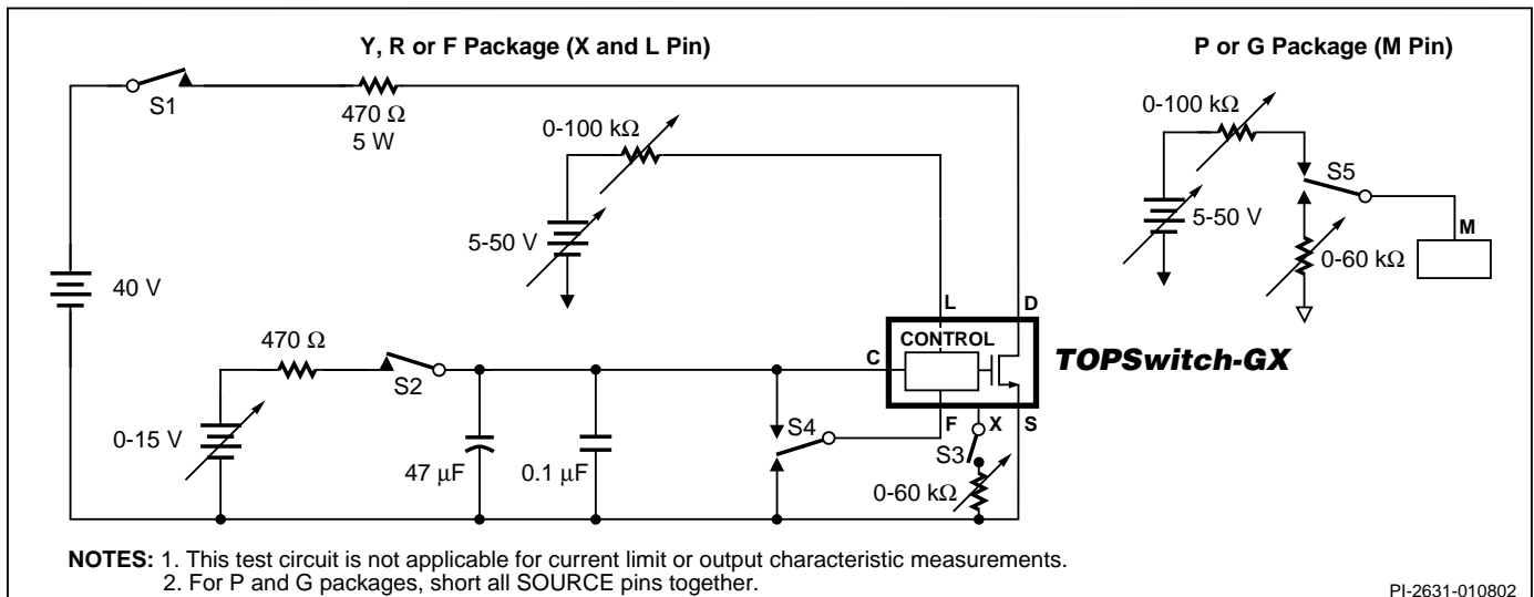
Figure 53. TOPSwitch-GX General Test Circuit.
