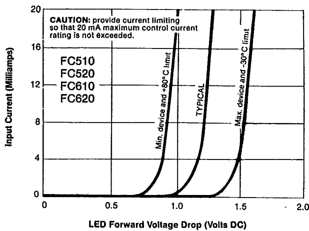
Figure 3. Input Characteristics (Current Controlled)
