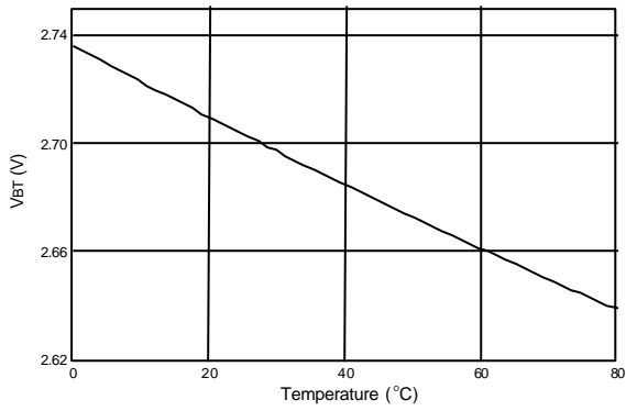
V_{BT} (high) Limit vs Temperature
