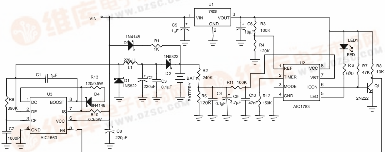
Battery Charge Circuit with Wide Input Voltage Range
