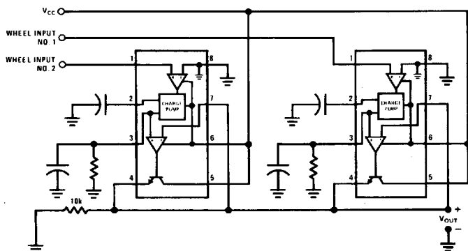
"Select-High" Circuit
