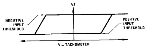
Tachometer Input Threshold Measurement
