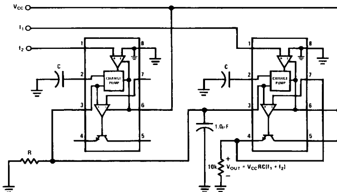
"Select-Average" Circuit
