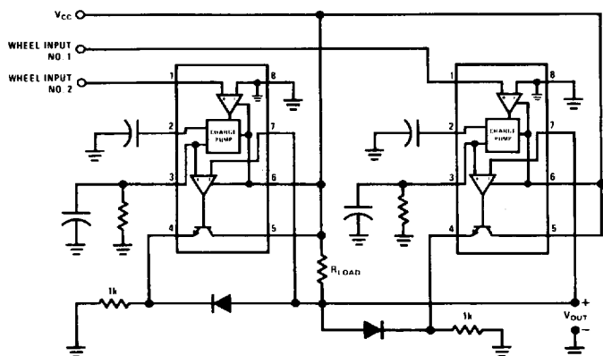
"Select-Low" Circuit
