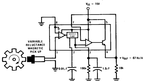
Minimum Component Tachometer
