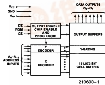
Figure 1. Block Diagram
