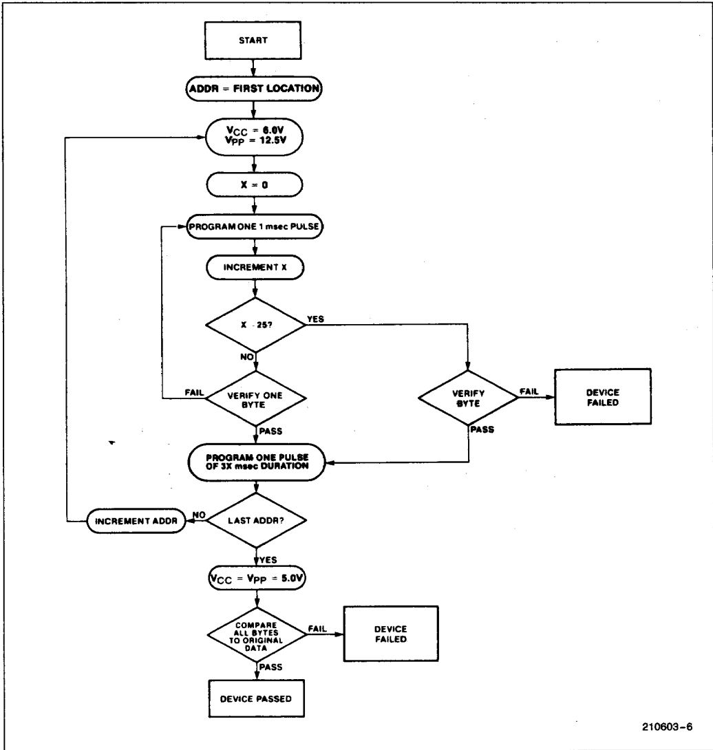
Figure 3. M27128A Intelligent Programming™ Flowchart
