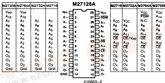
Figure 2. Pin Configurations
