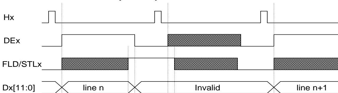
Figure 18: Stall Signal Timing
