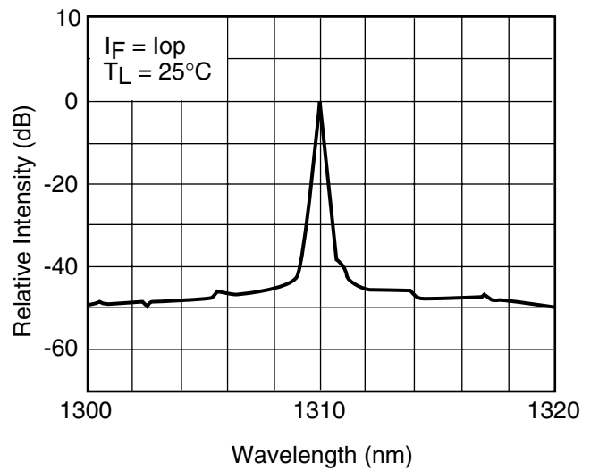
Fig. 4 Lasing Spectrum
