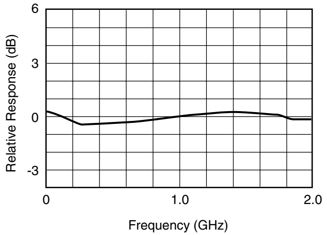
Fig. 6 Frequency Response
