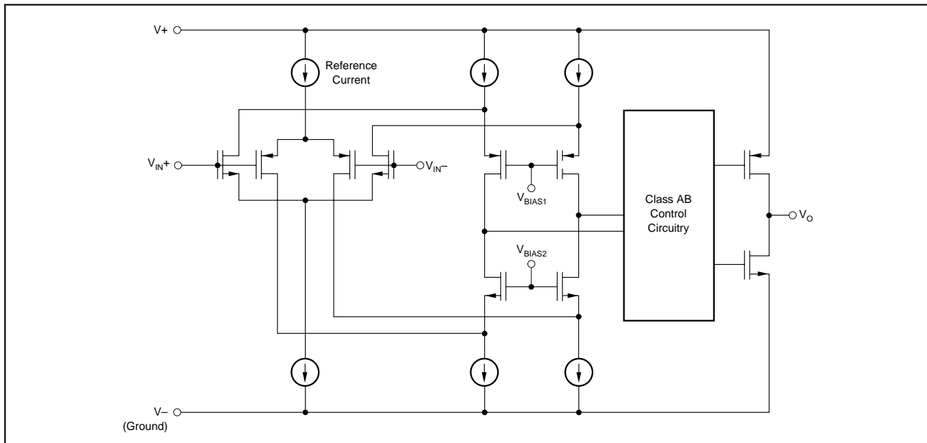
FIGURE 1. Rail-to-Rail Input and Output.
