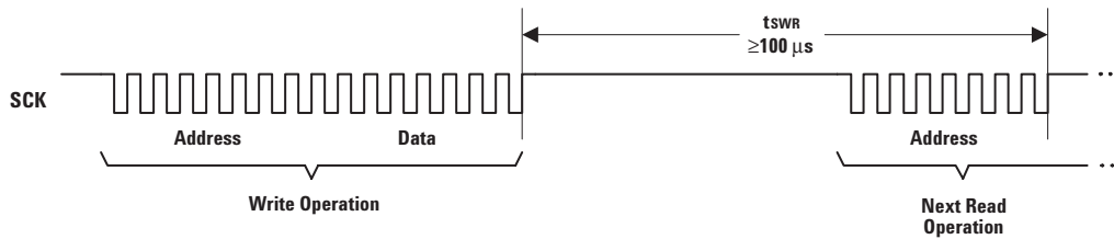
Figure 26. Timing between write and read commands.
