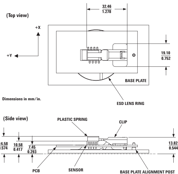
Figure 4. 2D assembly drawing of ADNS-2610 shown with the HLMP-ED80 (top and side view).
