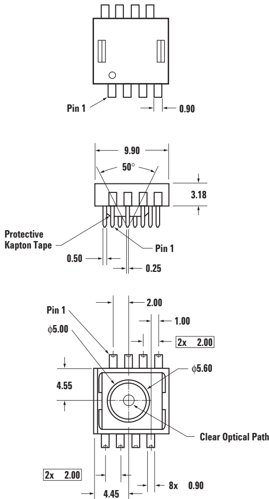
Figure 2. Package outline drawing.
