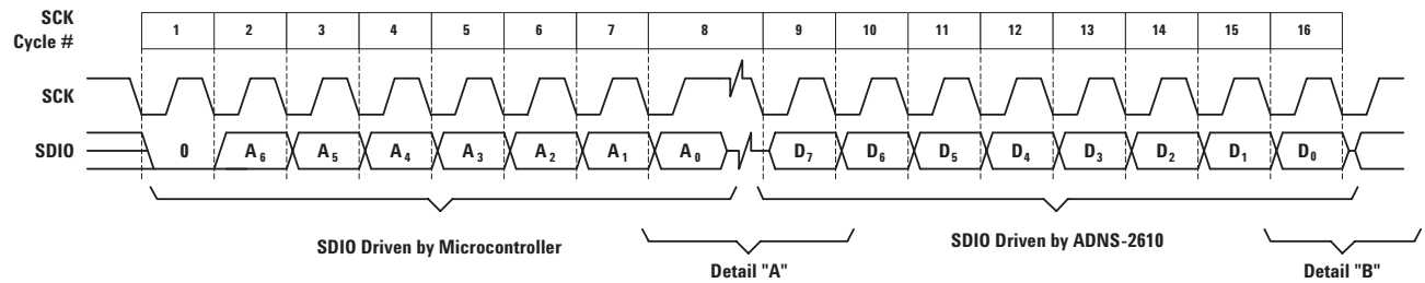
Figure 21. Read operation.
