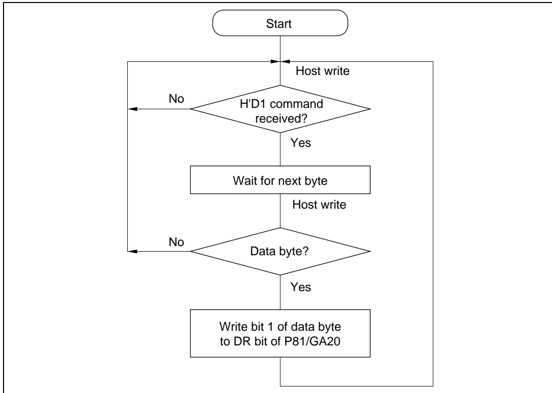
Figure 17.2 GA20 Output
