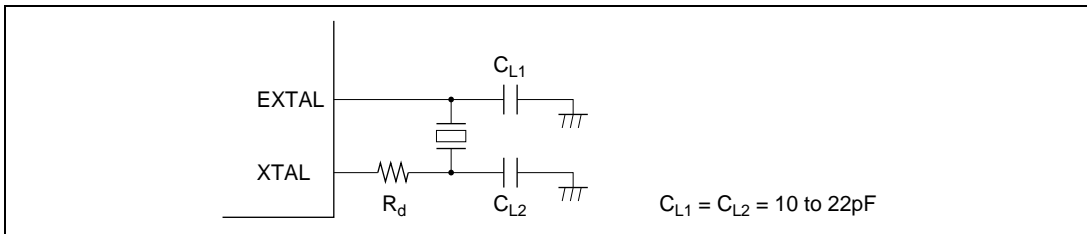
Figure 22.2 Connection of Crystal Resonator (Example)
