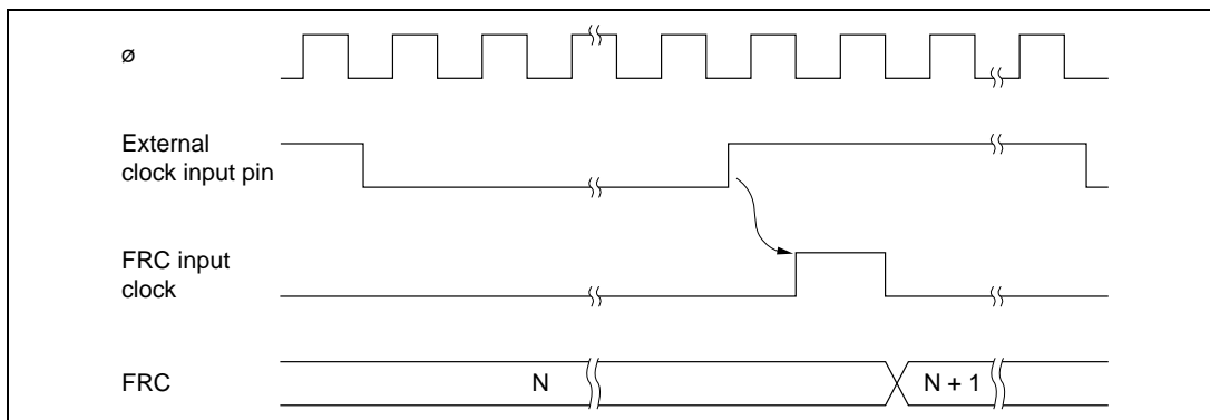
Figure 11.4 Increment Timing with External Clock Source
