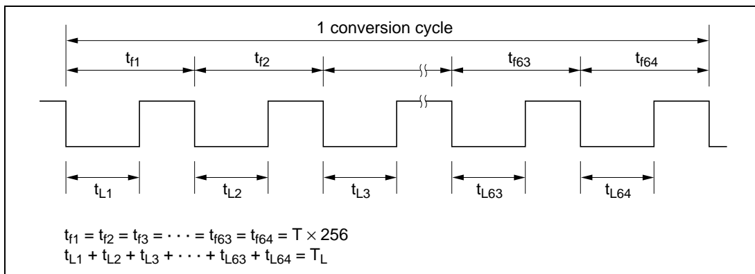
Figure 10.4 (2) Output Waveform
