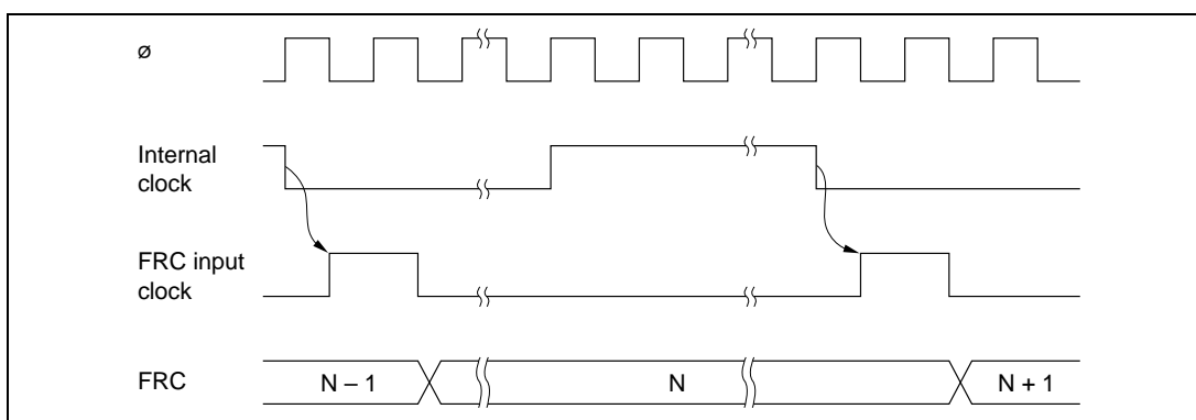
Figure 11.3 Increment Timing with Internal Clock Source
