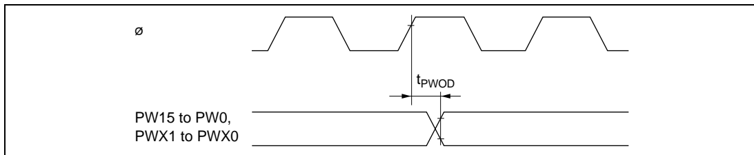
Figure 24.20 PWM, PWMX Output Timing
