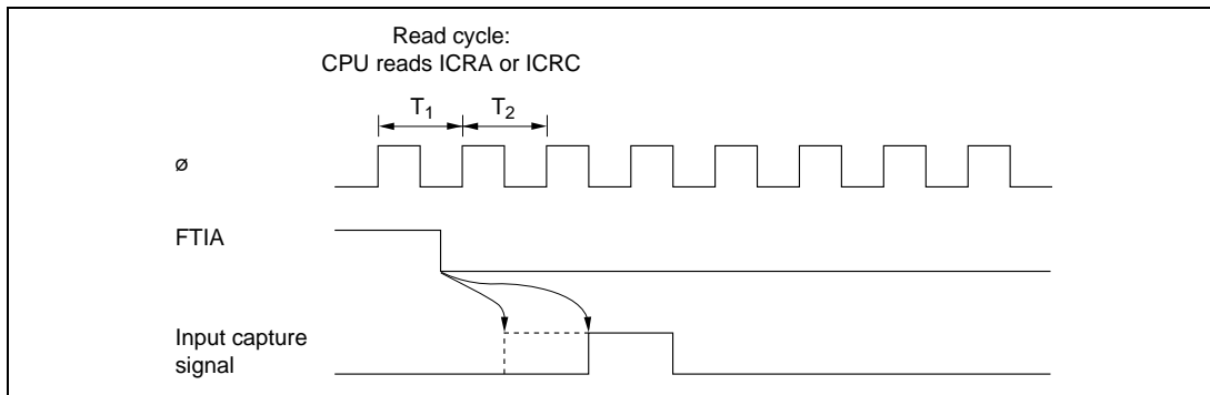
Figure 11.10 Buffered Input Capture Timing (Input Capture Input when ICRA or ICRC is Read)
