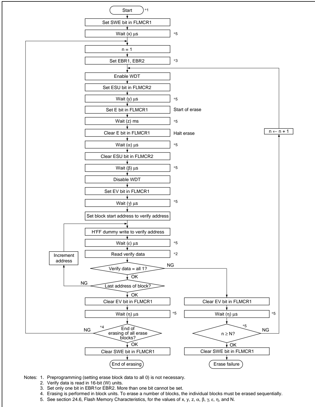
Figure 21.13 Erase/Eraser-Verify Flowchart (Single-Block Erase)
