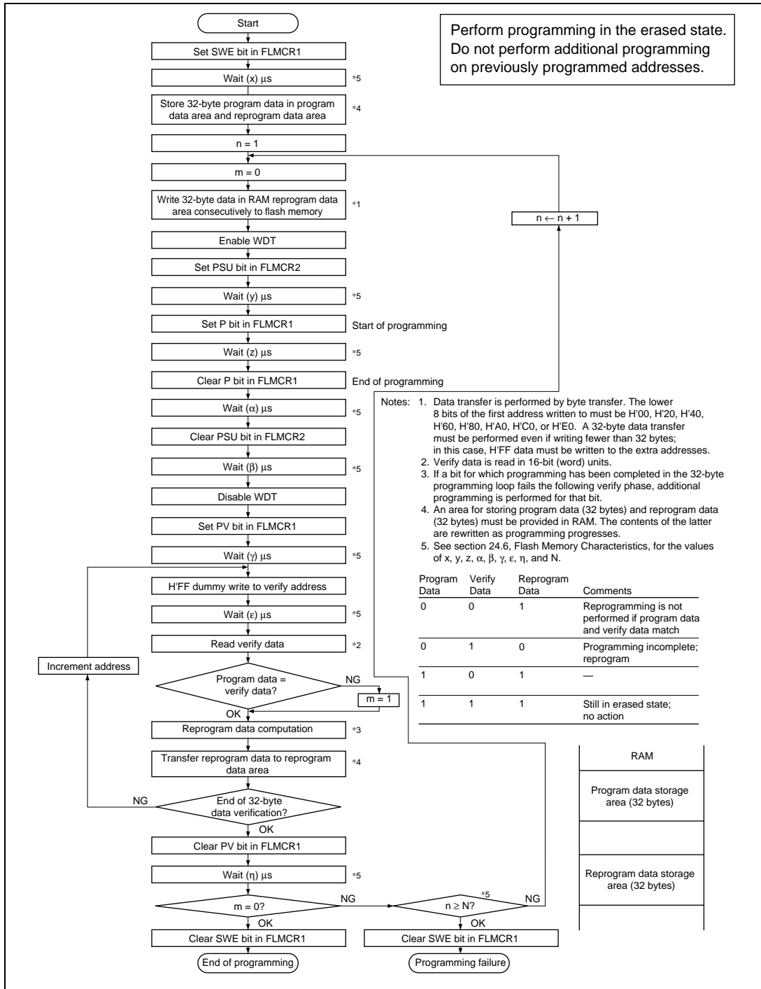
Figure 21.12 Program/Program-Verify Flowchart
