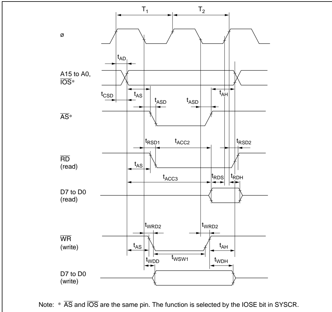
Figure 24.9 Basic Bus Timing (Two-State Access)
