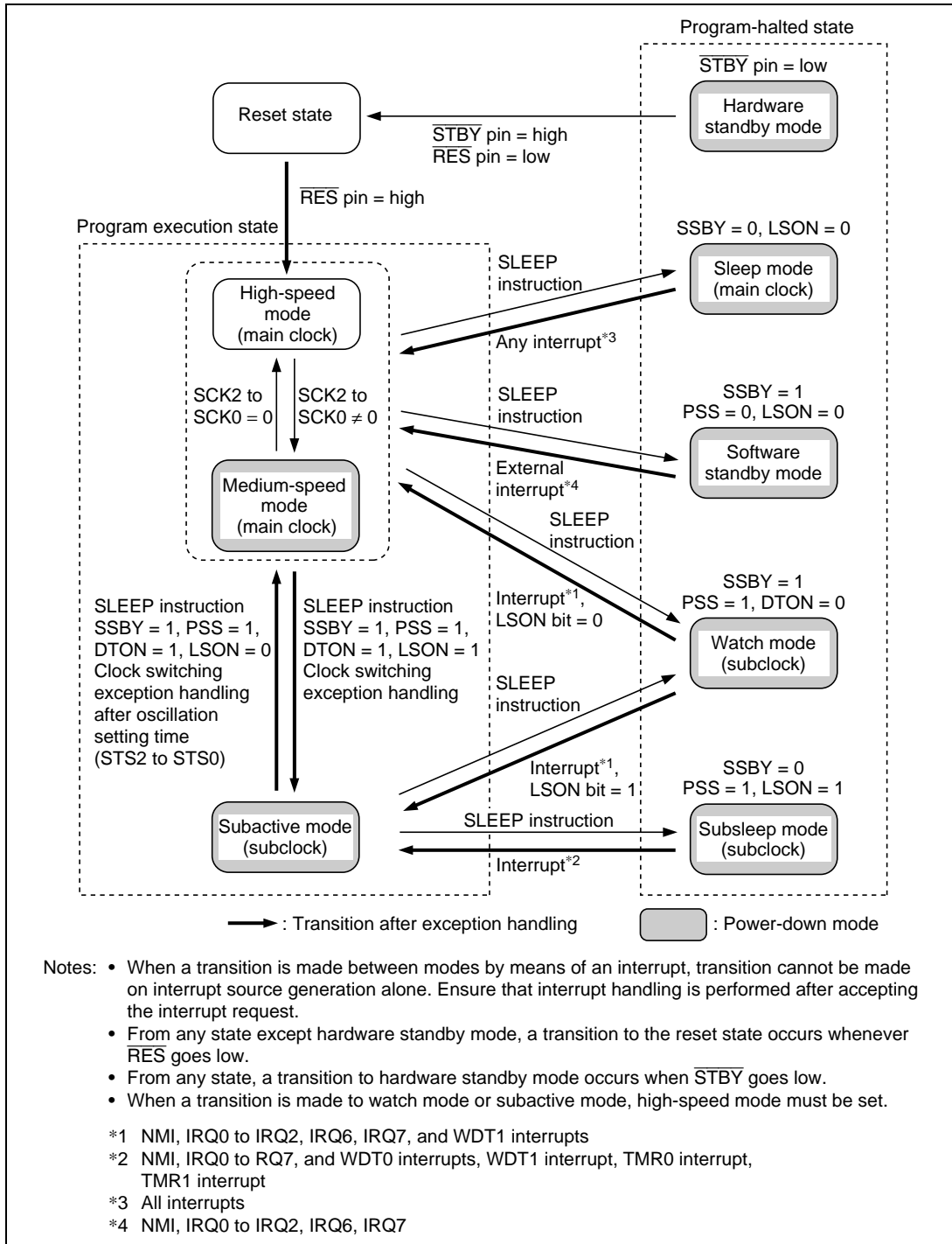
Figure 23.1 Mode Transitions
