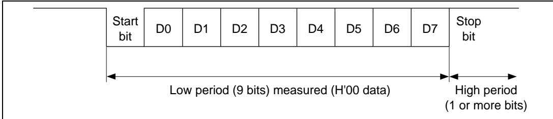
Figure 21.9 RxD1 Input Signal when Using Automatic SCI Bit Rate Adjustment
