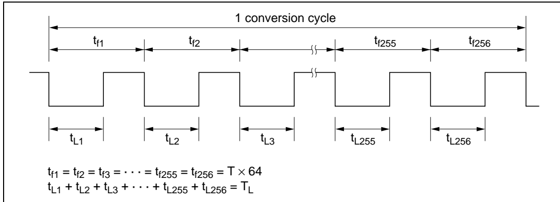
Figure 10.4 (1) Output Waveform
