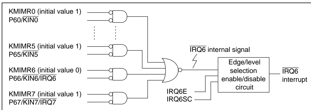
Figure 5.2 Relationship between Interrupts IRQ6, Interrupts \overline{KIN7} to \overline{KIN0} , and Registers KMIMR
