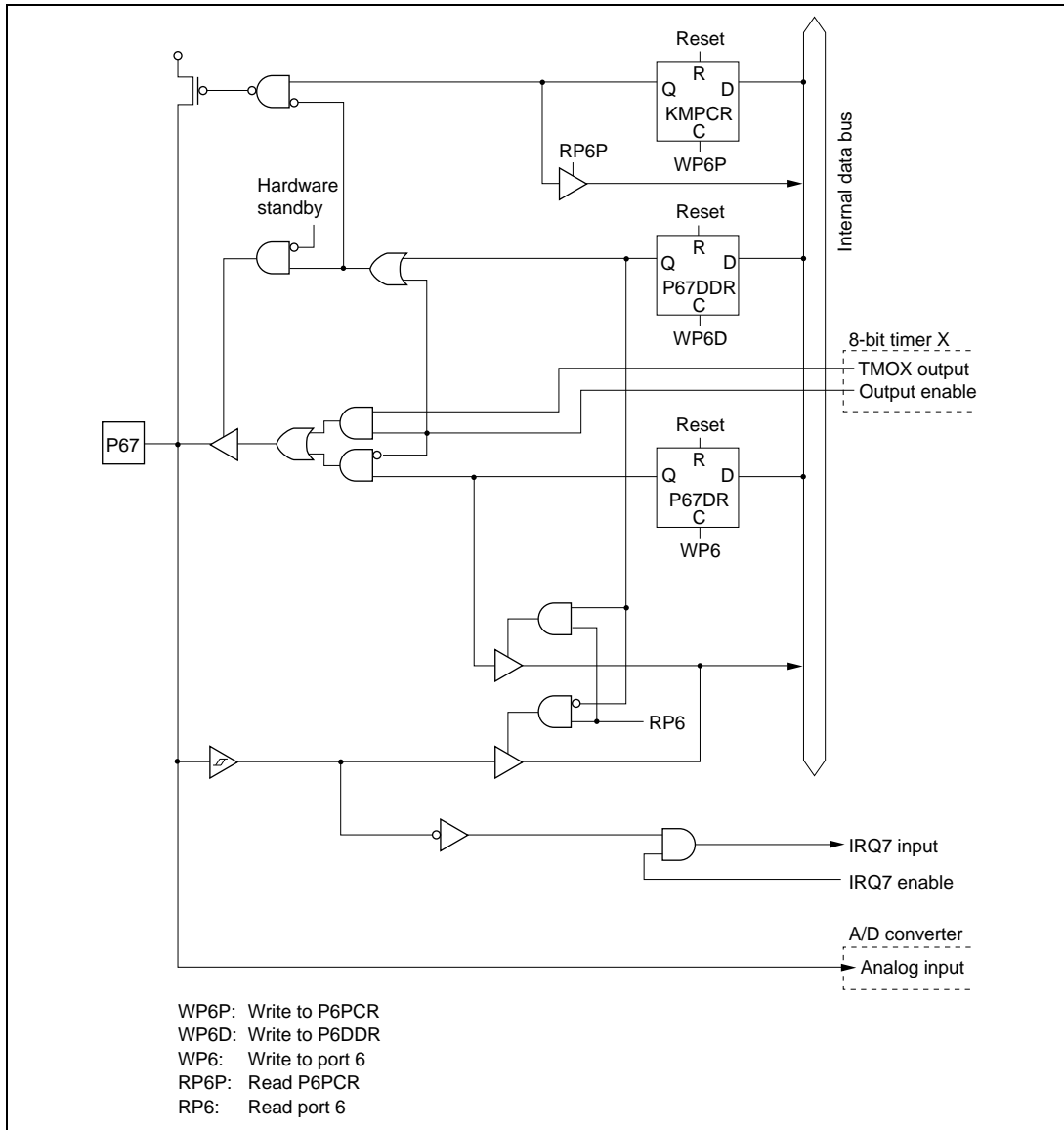
Figure C.20 Port 6 Block Diagram (Pin P67)
