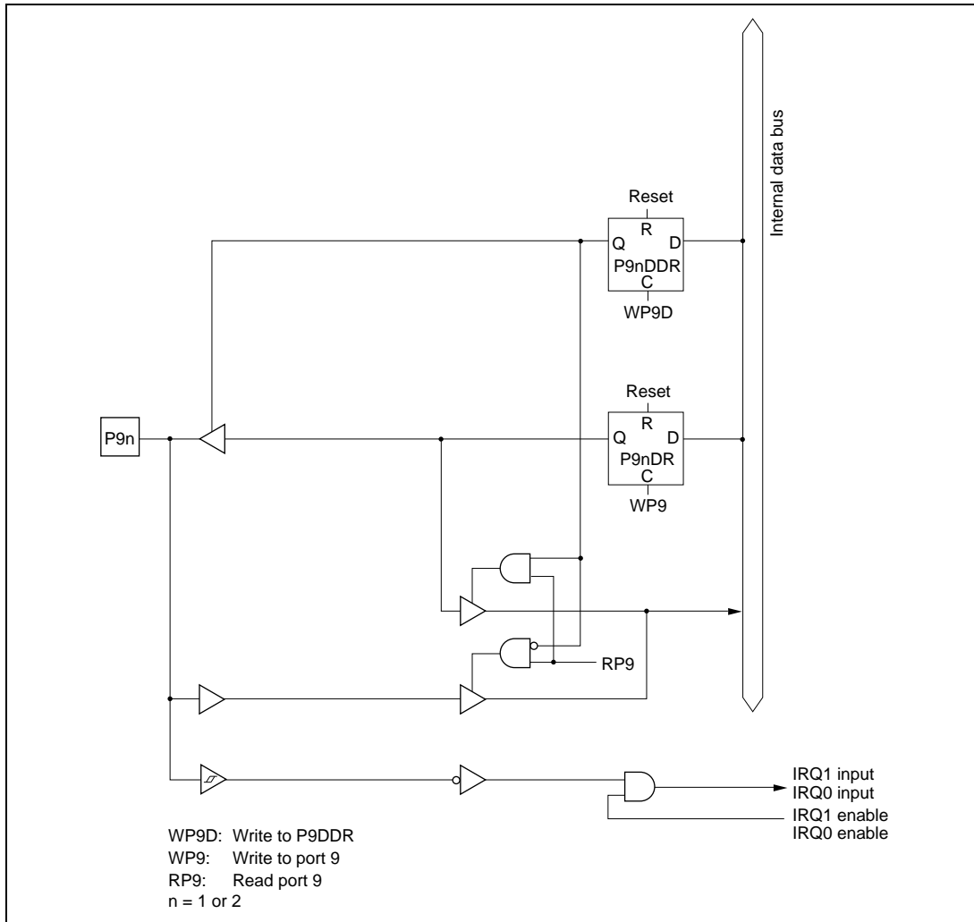
Figure C.30 Port 9 Block Diagram (Pins P91, P92)
