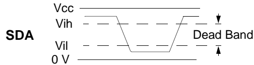
Figure 12. SDA/SCL Levels
