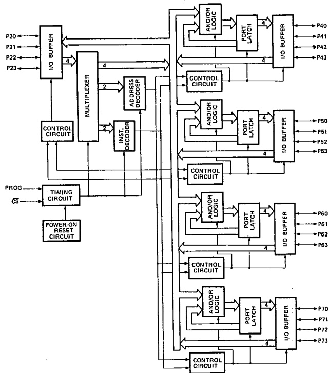
Fig. 3 - BLOCK DIAGRAM
