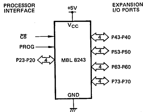
Fig. 2 - LOGIC SYMBOL
