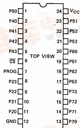
Fig. 1 - PIN ASSIGNMENT
