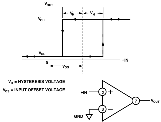
Figure 14. Hysteresis Definitions (N, Q Package Pinout)
