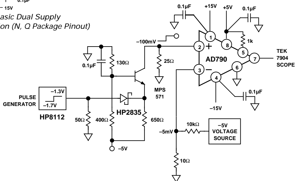
Figure 2. Response Time Test Circuit (N/O Package Pinout)
