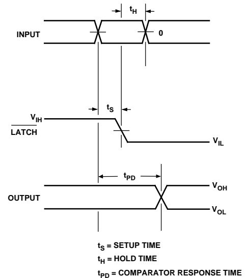
Figure 12. Latch Timing
