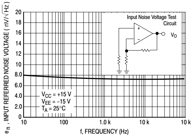
Figure 28. Input Referred Noise Voltage versus Frequency
