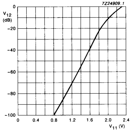
Fig.8 Volume control characteristics.
