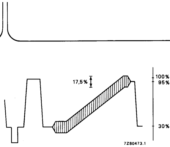
Fig.2 Video output signal.
