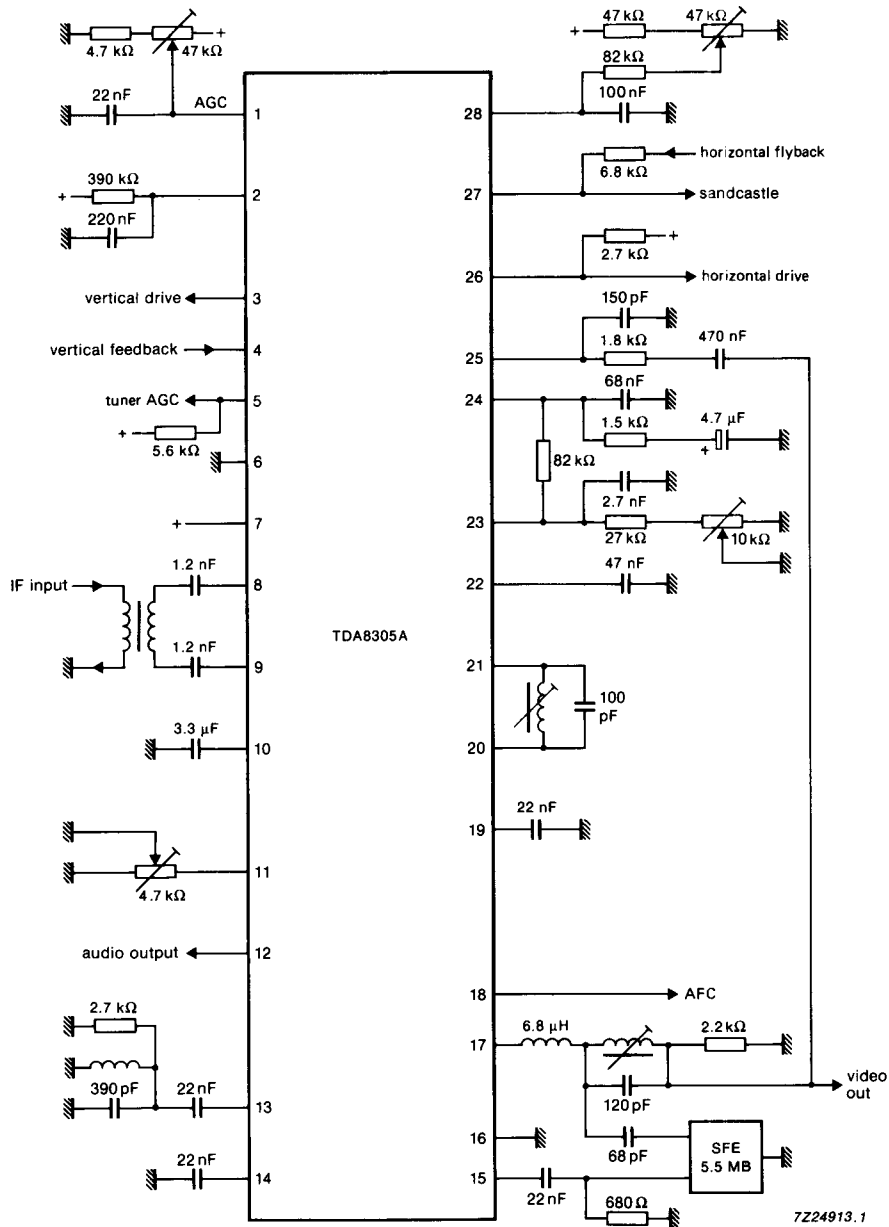
Fig.11 Application diagram.
