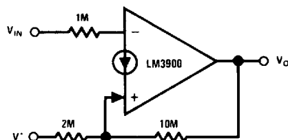
Schmitt-Trigger
