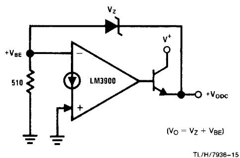
Voltage Regulator
