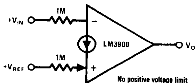
Comparator
