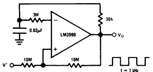
Square-Wave Oscillator
