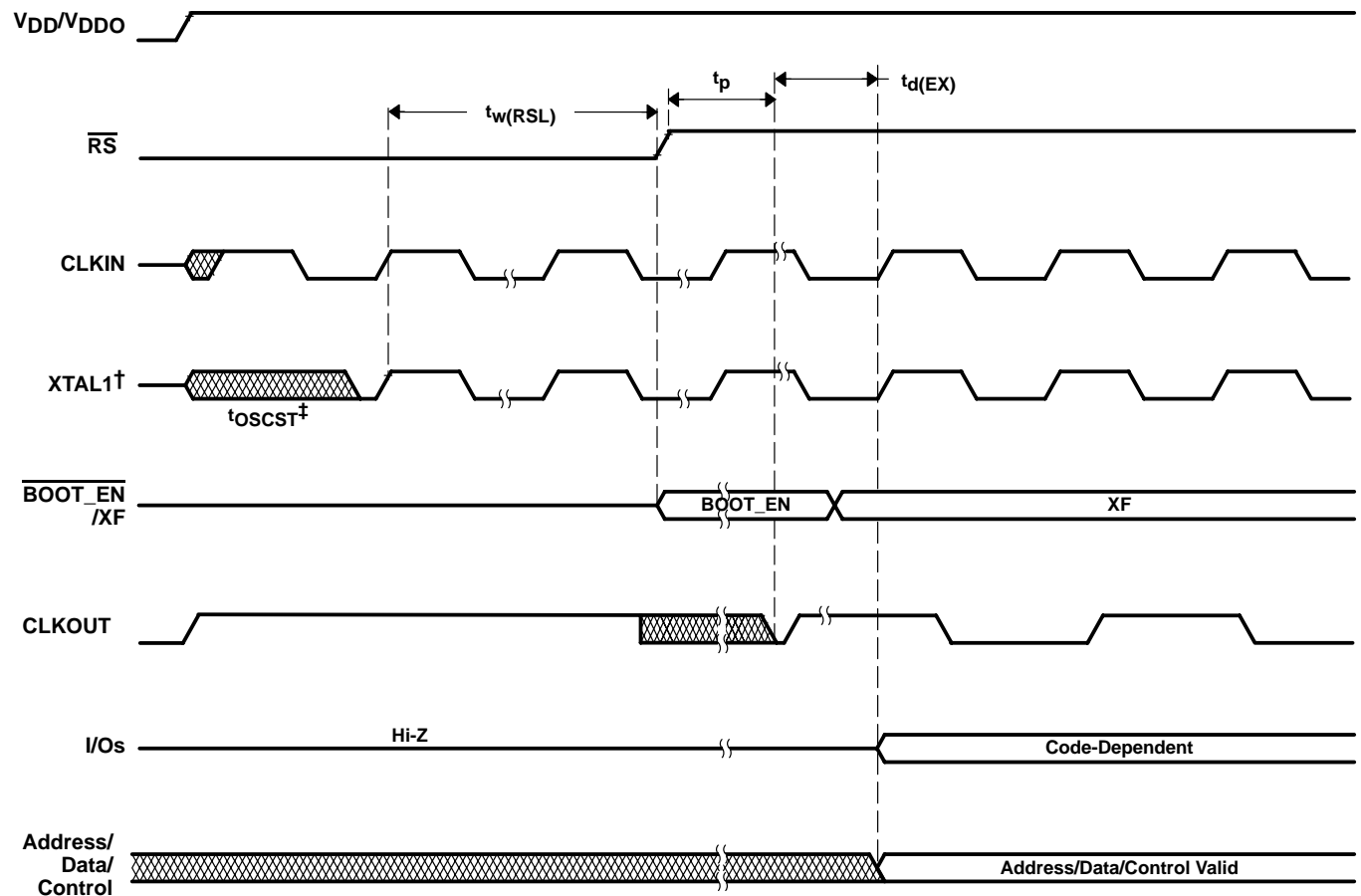
Figure 26. Power-on Reset
