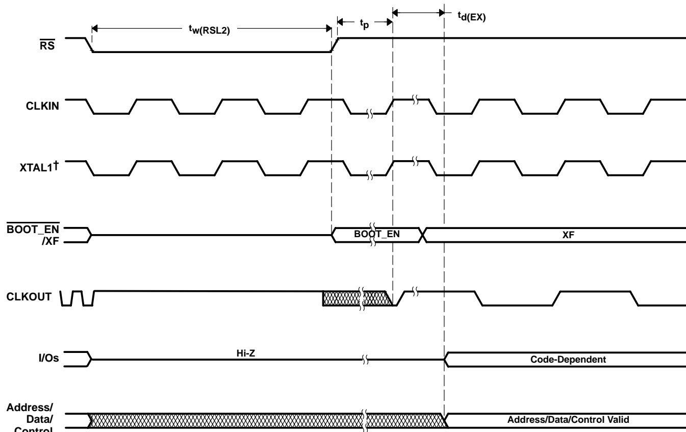
Figure 27. Warm Reset
