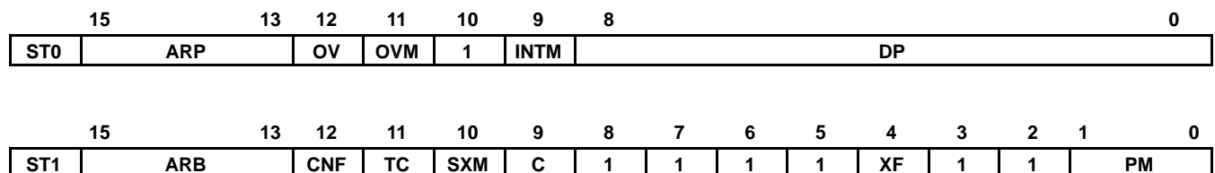
Figure 9. Organization of Status Registers ST0 and ST1
