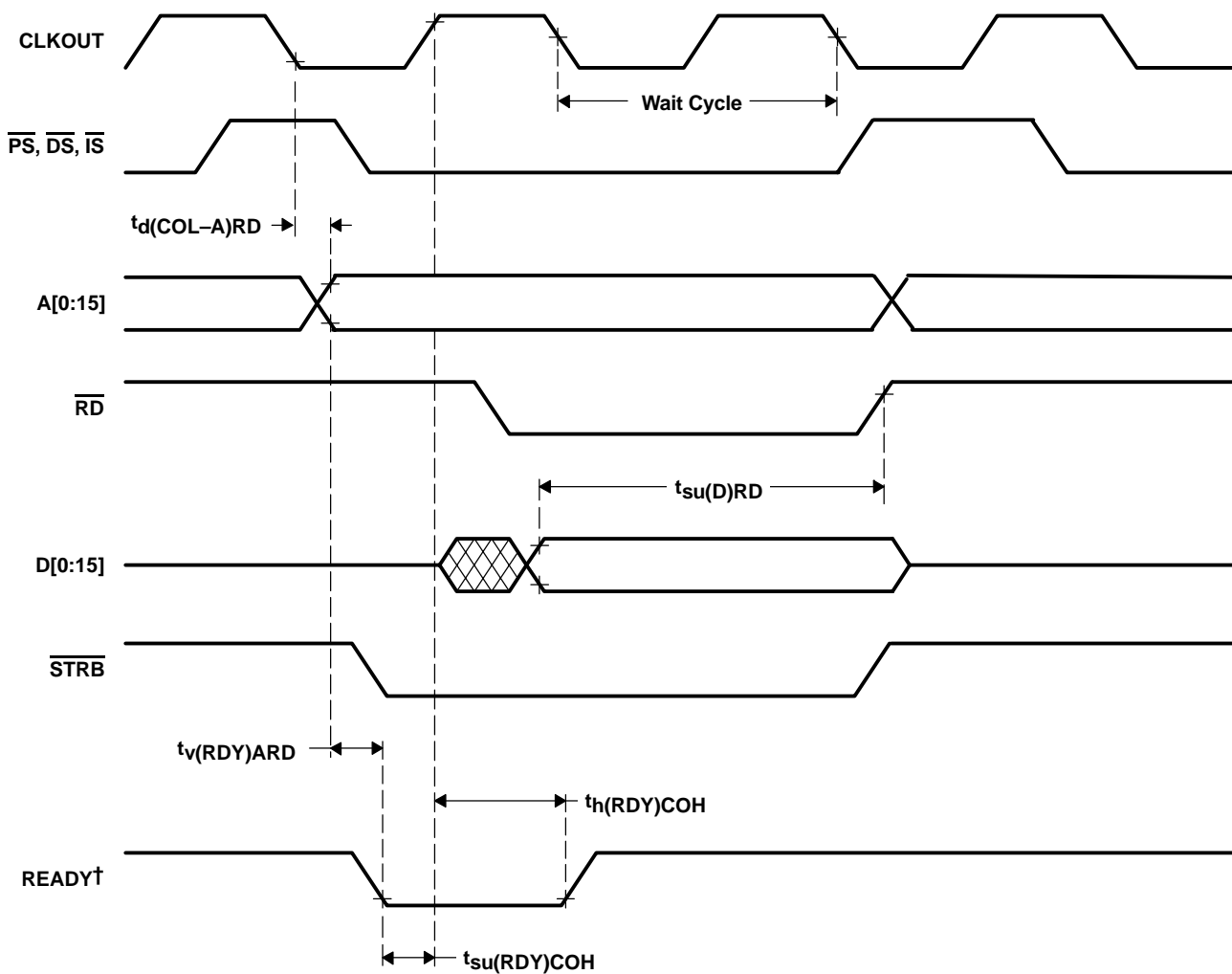
Figure 46. Ready-on-Read Timings
