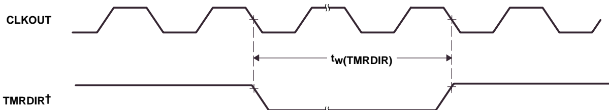
Figure 35. TMRDIR Timing
