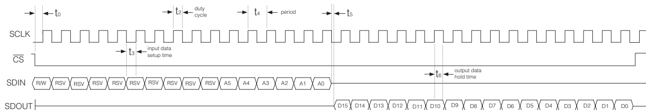
Figure 18 GSPI Read Mode Timing
