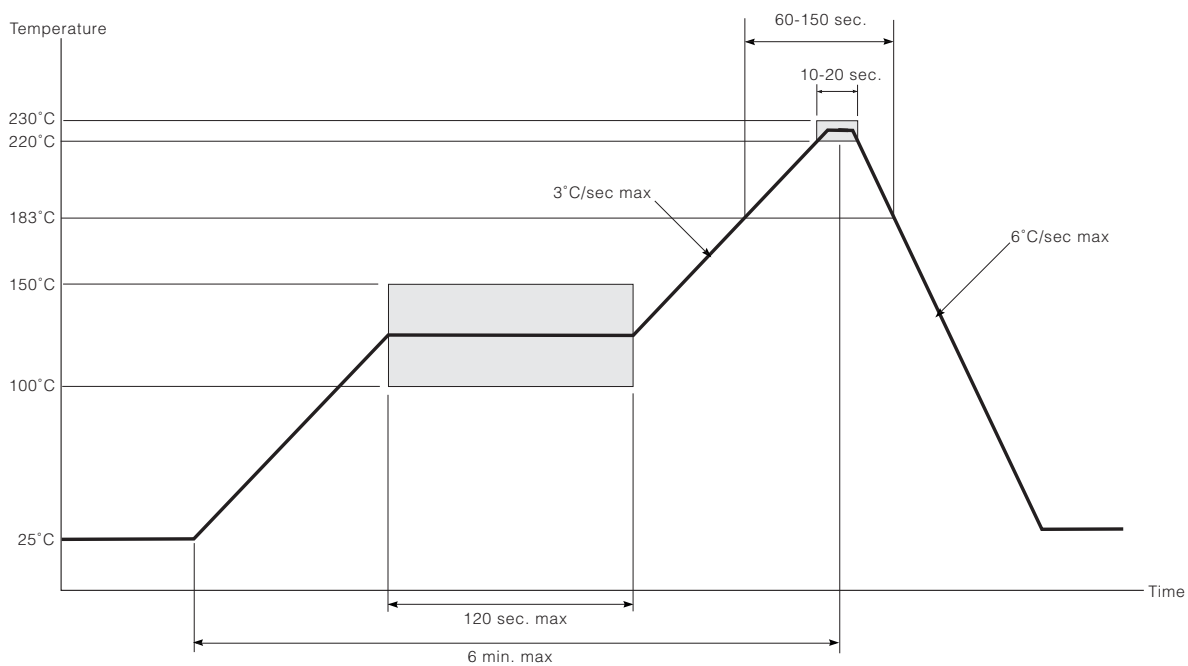
Figure 1 Reflow Solder Profile
