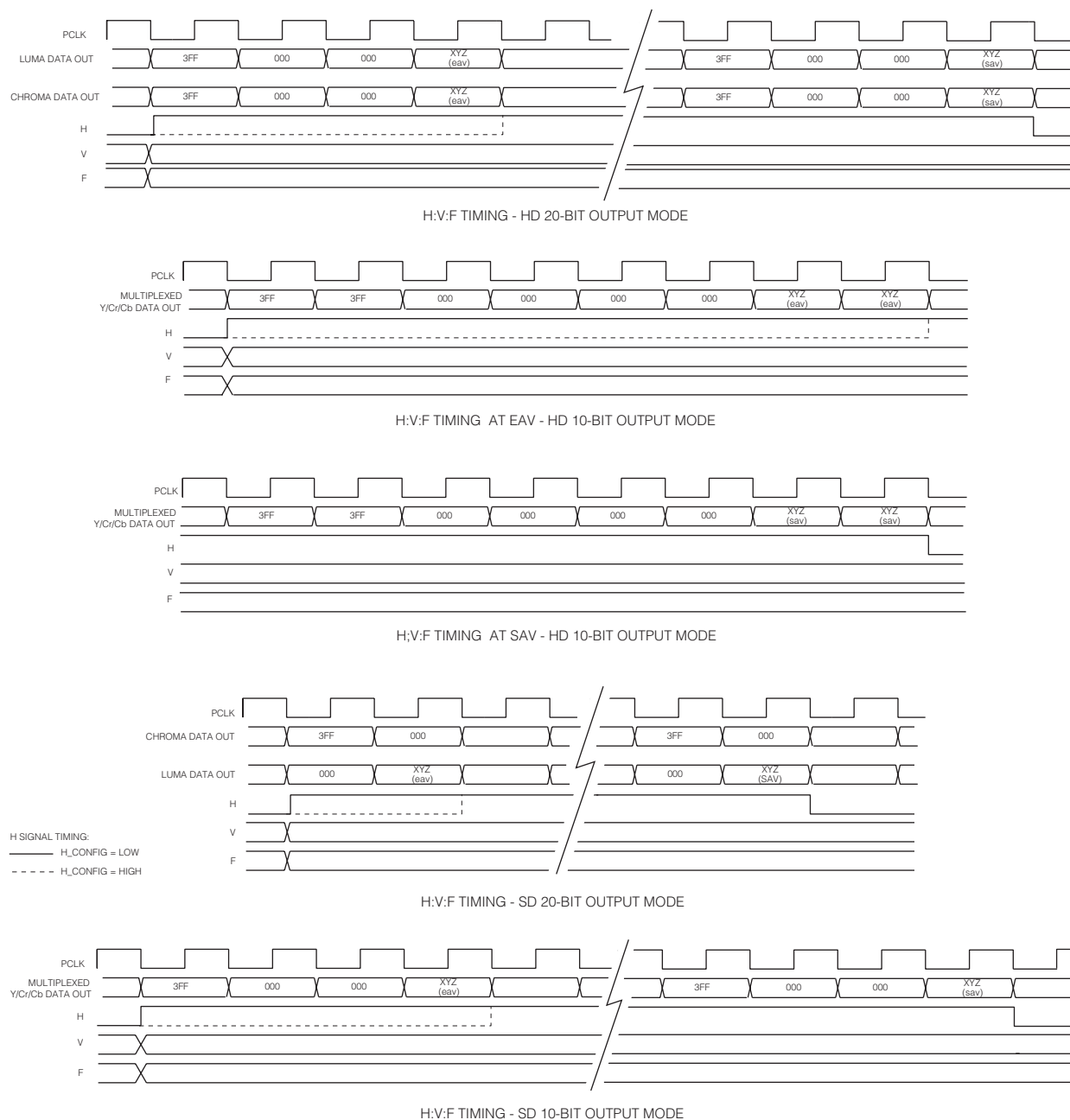
Figure 9 H, V, F Timing
