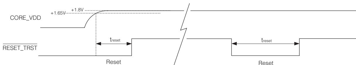
Figure 22 Reset Pulse
