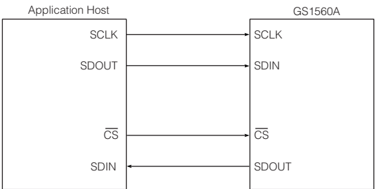
Figure 15 Gennum Serial Peripheral Interface (GSPI)
