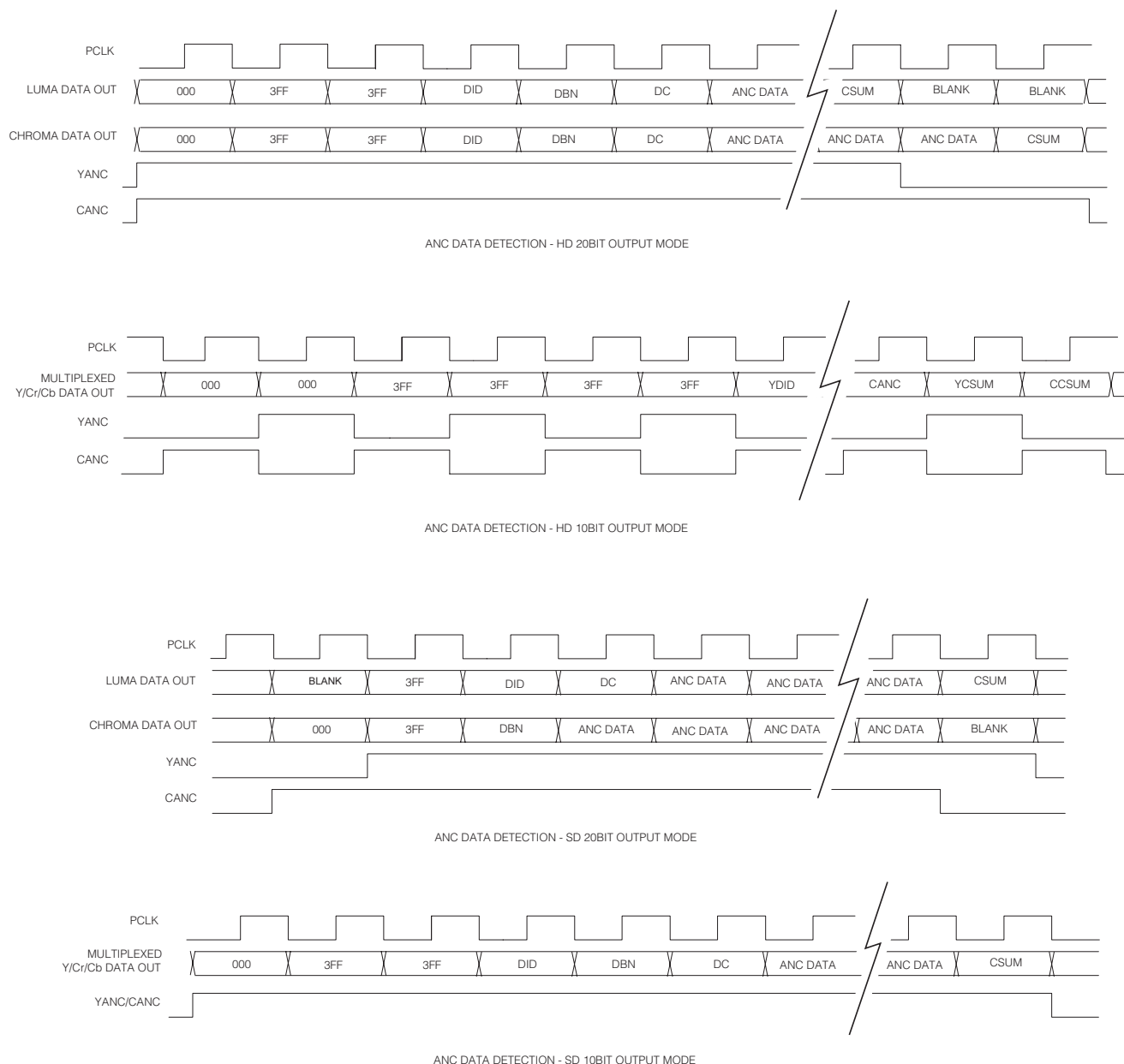
Figure 12 YANC and CANC Output Signal Timing
