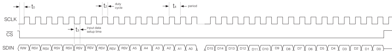
Figure 19 GSPI Write Mode Timing
