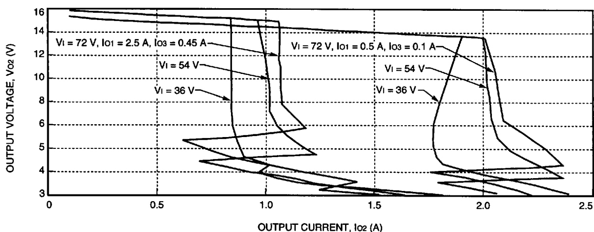
Figure 12. DW025ACL Typical 15 V Output Characteristics
