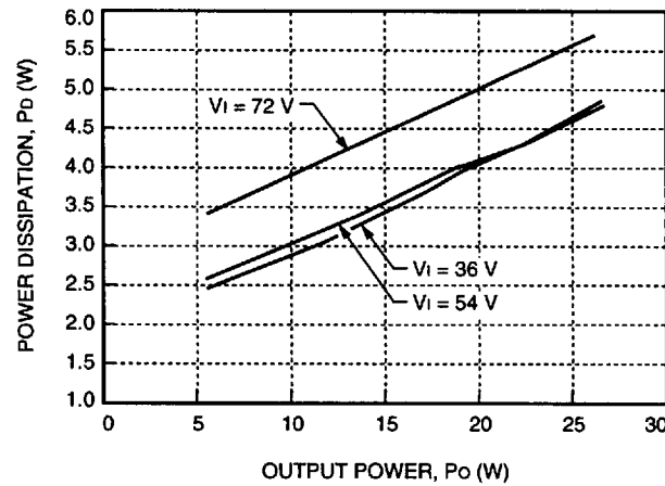
Figure 24. DW025ACL Fixed Losses, P_p
