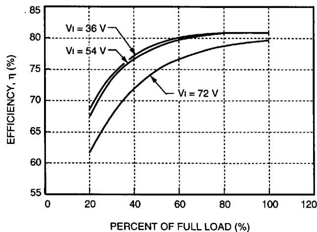
Figure 12. DW025ACL Typical 15 V Output Characteristics
