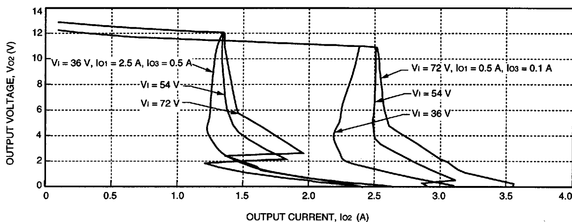
Figure 10. DW025ABK Typical 12 V Output Characteristics
