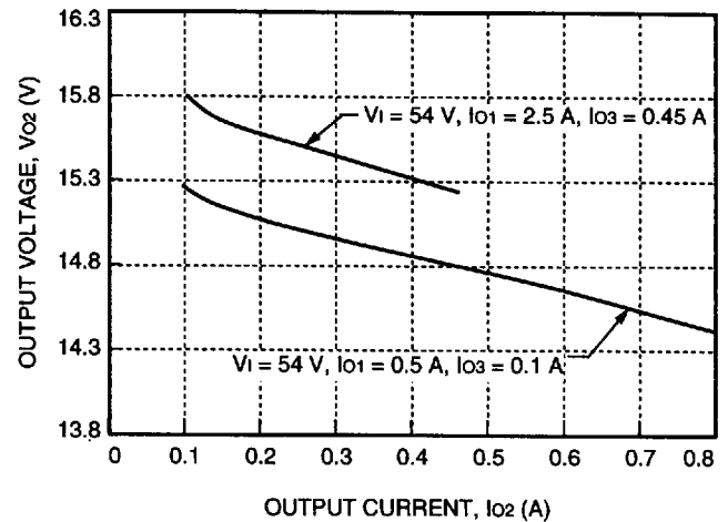
Figure 7. DW025ACL Typical Load Regulation
