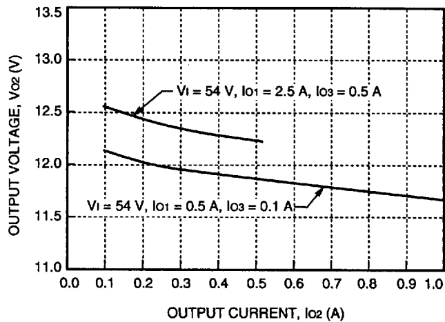
Figure 5. DW025ABK Typical Load Regulation
