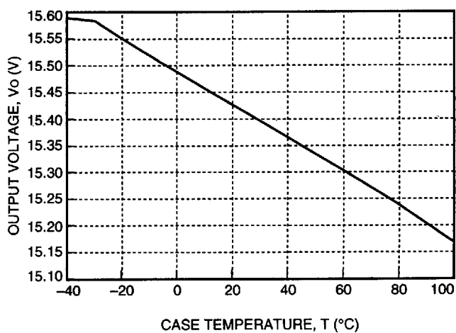
Figure 4. DW025 Triple Output-Series Typical Output Voltage Variation of 15 V Output Over Ambient Temperature Range
