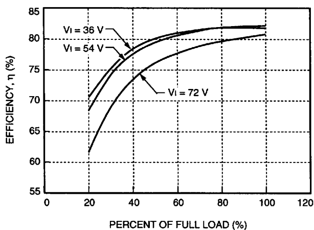
Figure 13. DW025ABK Typical Converter Efficiency
