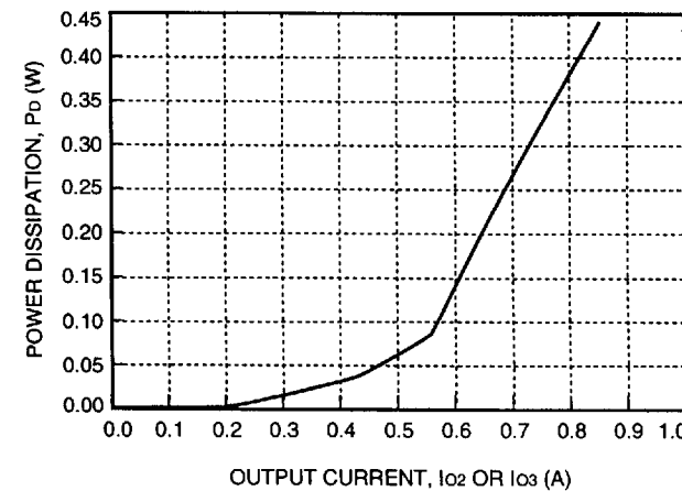
Figure 26. DW025ABK, Losses Associated with \pm 12 V Output, P_{s2}/P_{s3}
