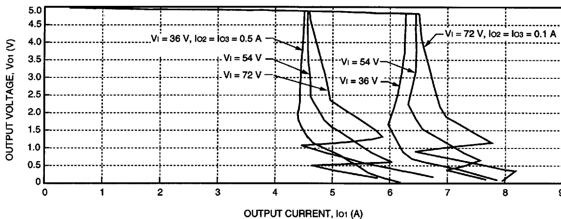
Figure 9. DW025ABK Typical 5 V Output Characteristics
