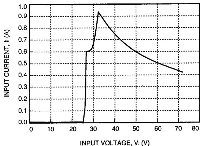
Figure 1. DW025 Triple Output-Series Typical Input Characteristics
