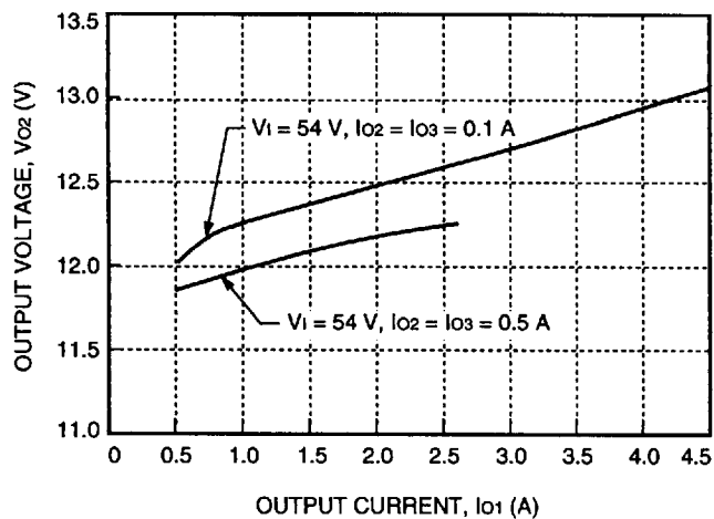
Figure 6. DW025ABK Typical Cross Regulation with Respect to I_{01}
