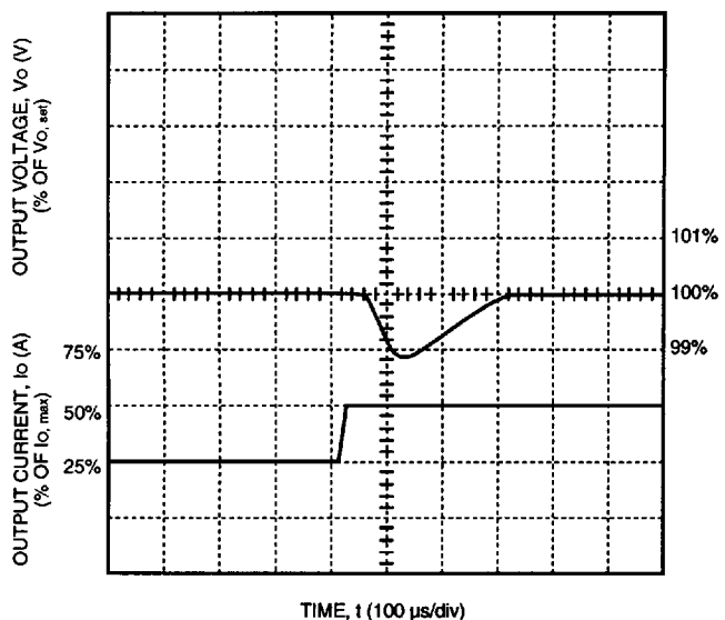
Figure 16. DW025 Triple Output-Series Typical Output Voltage for a Step Load Change from 25% to 50% of Full Load on Output 1
