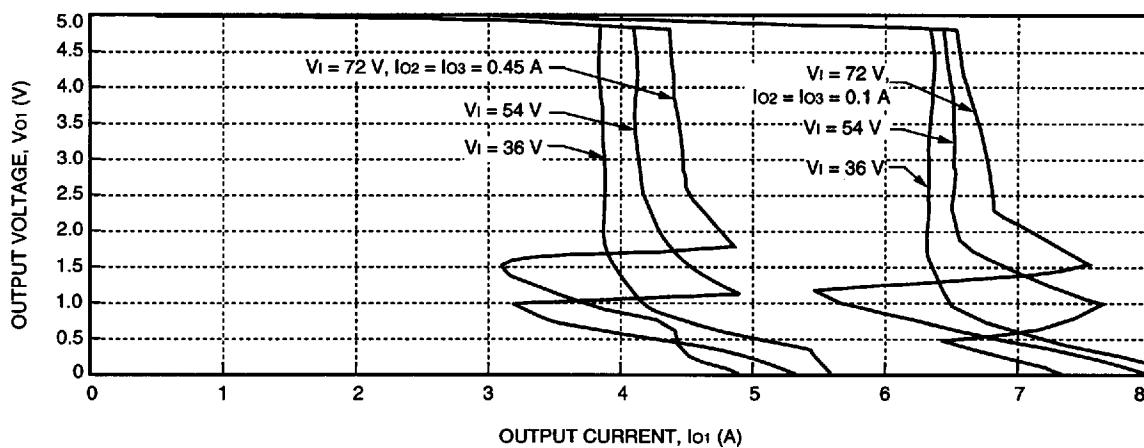
Figure 11. DW025ACL Typical 5 V Output Characteristics
