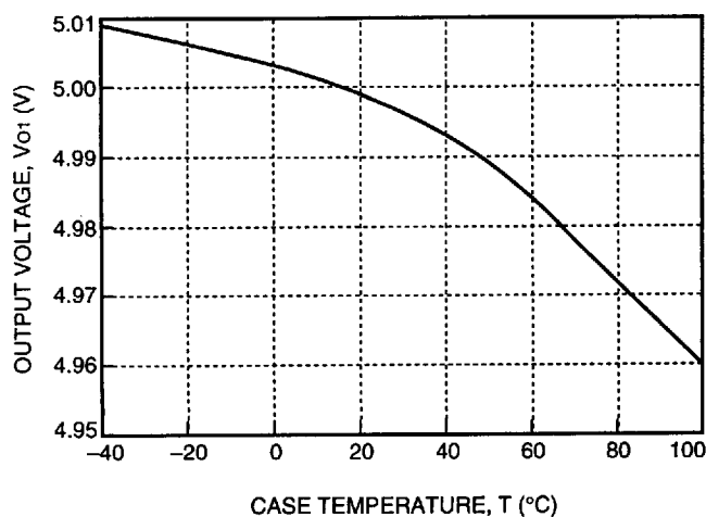
Figure 2. DW025 Triple Output-Series Typical Output Voltage Variation of 5 V Output Over Ambient Temperature Range
