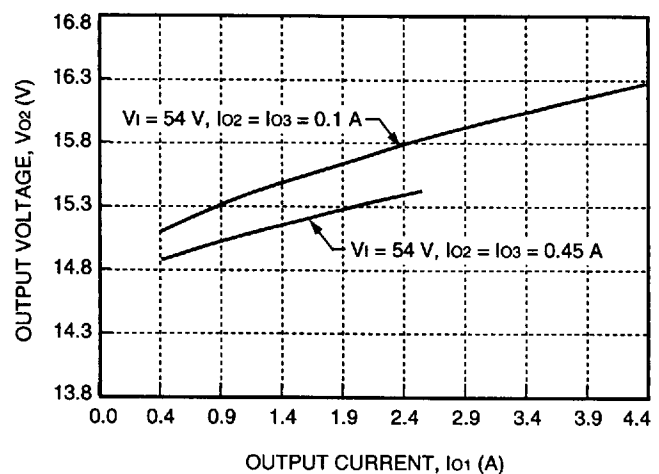
Figure 8. DW025ACL Typical Cross Regulation with Respect to I_{01}
