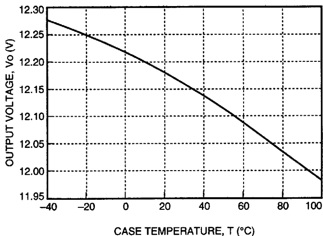
Figure 3. DW025 Triple Output-Series Typical Output Voltage Variation of 12 V Output Over Ambient Temperature Range
