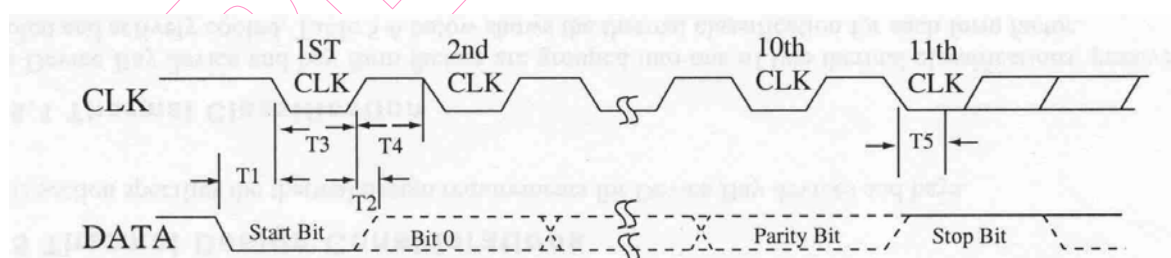
Fig 3. Keyboard output data timings
