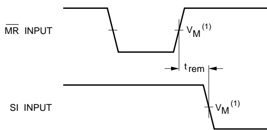
Fig.16 Waveform showing the \overline{MR} input to SI input removal time.
