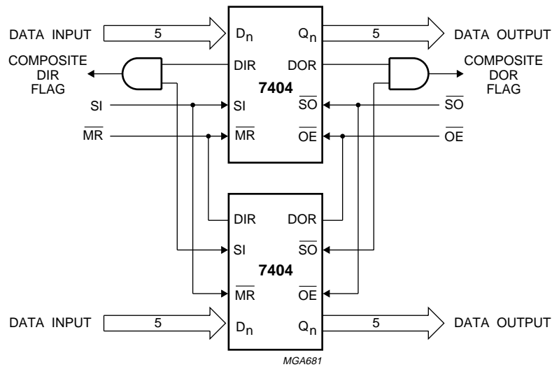
Fig.19 Expanded FIFO for increased word length; 64 words \times 10 bits.
