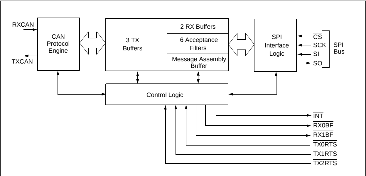
FIGURE 1-1: Block Diagram
