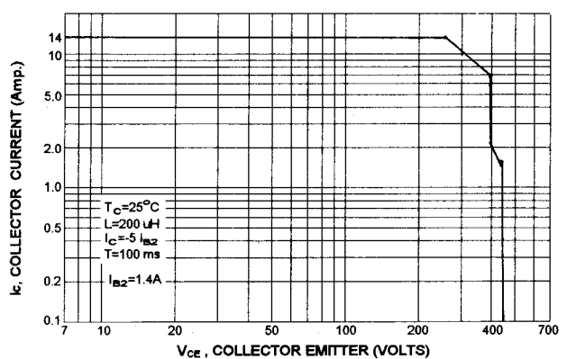
REVERSE BIASE SAFE OPERATING AREA
