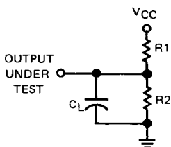
LOAD CIRCUIT FIGURE 2
