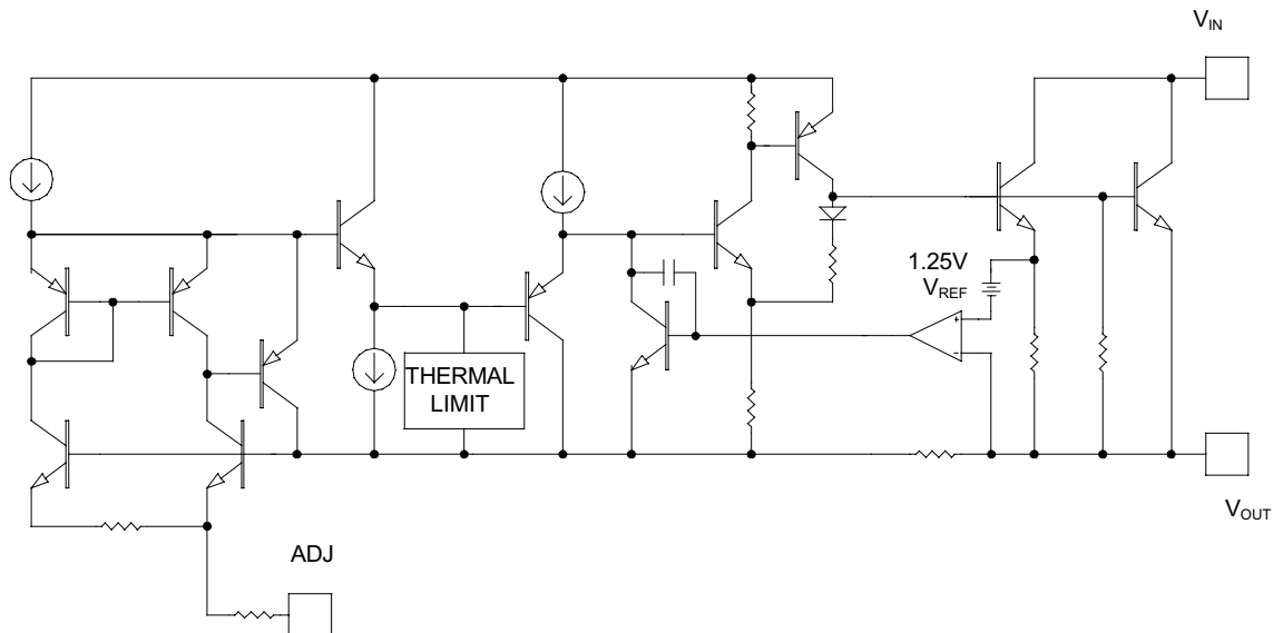
AMC7587-ADJ circuit schematic
