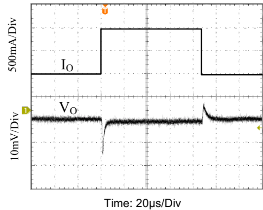
Load Transient Response with I_O=1A
