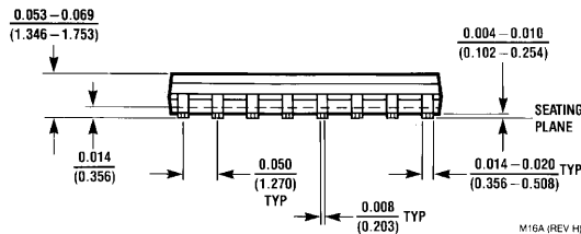
16-Lead Small Outline Molded Package (M) Order Number DM74LS190M, DM74LS191M NS Package Number M16A
