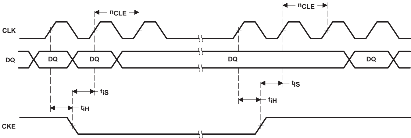
Figure 17. CLK-Suspend Operation
