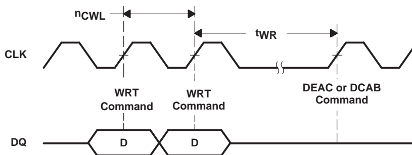
Figure 14. Write Followed By Deactivate
