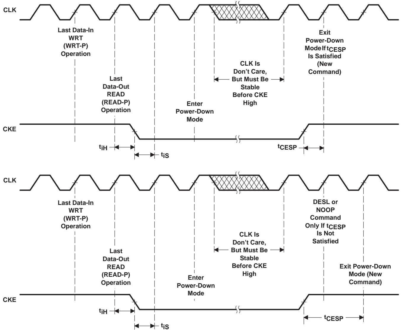
Figure 18. Power-Down Operation
