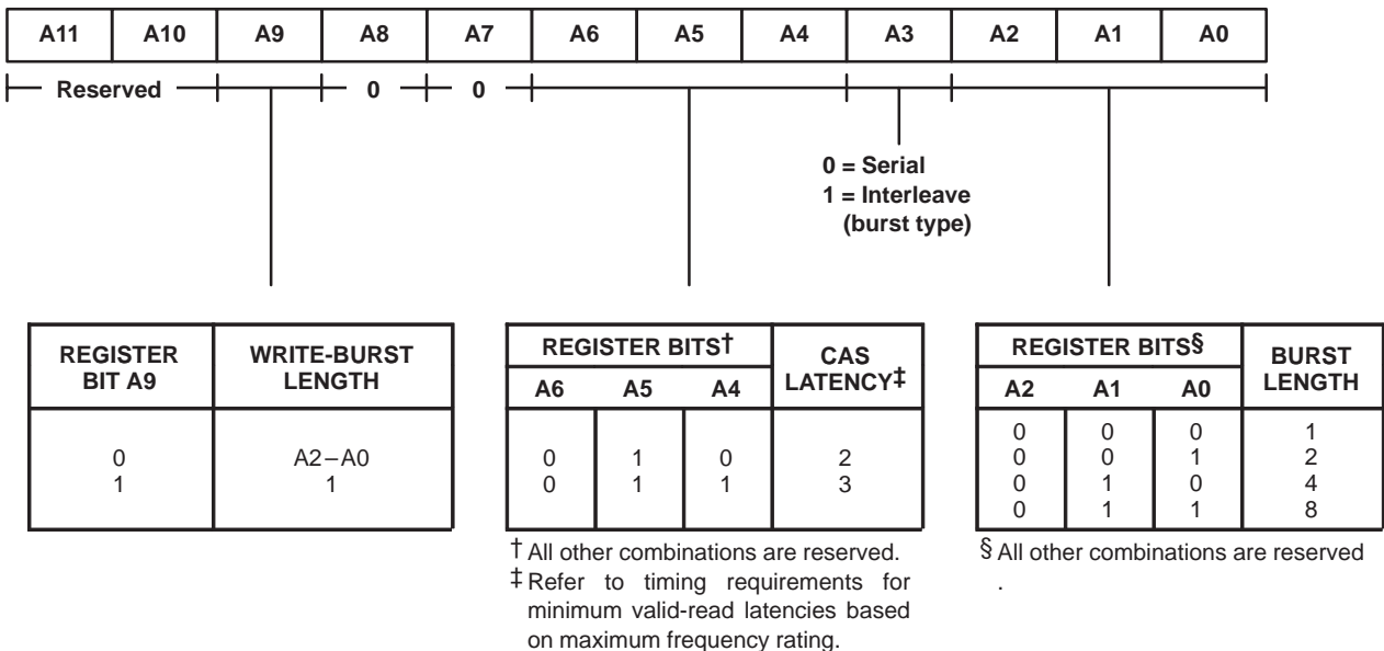
Figure 1. Mode-Register Programming
