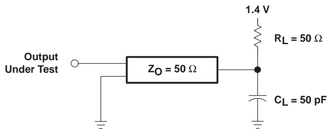
Figure 8. LVTTTL-Load Circuit
