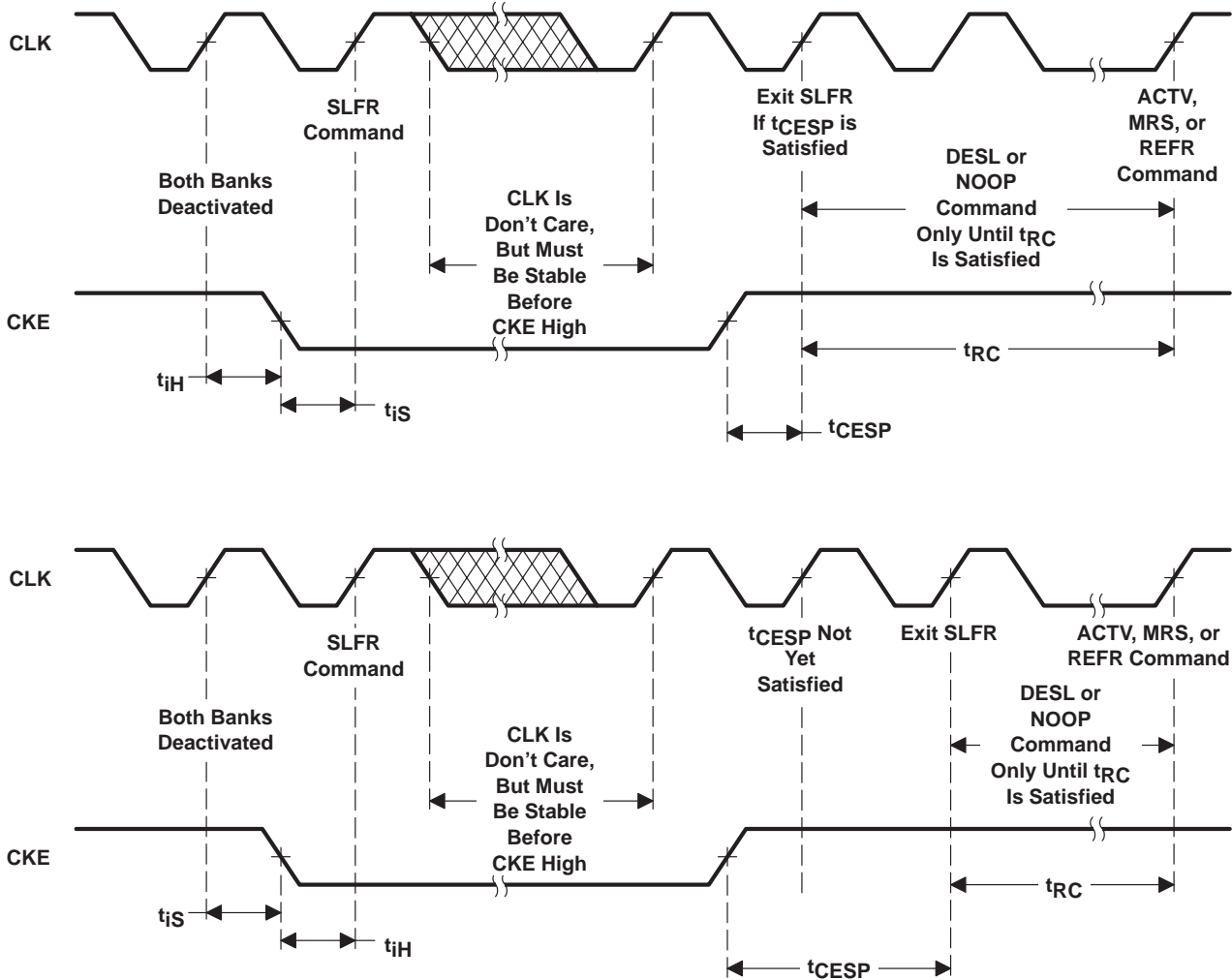
Figure 19. Self-Refresh Operation
