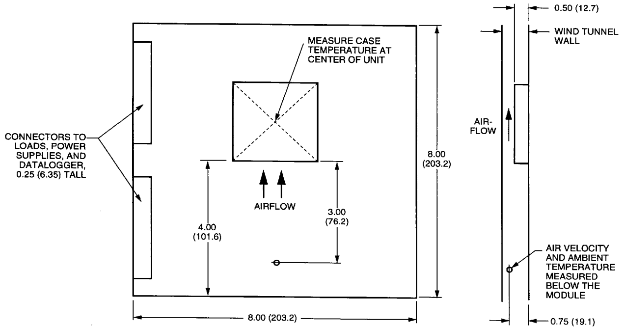
Figure 19. Thermal Test Setup
