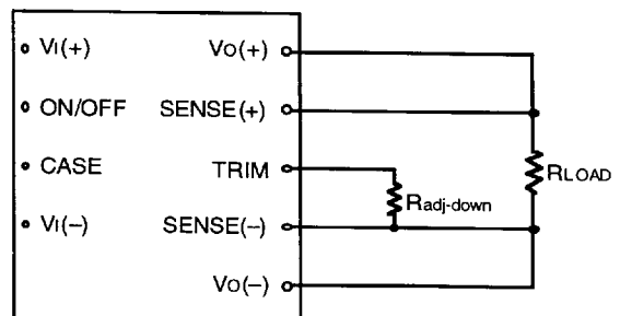
Figure 17. Circuit Configuration to Decrease Output Voltage
