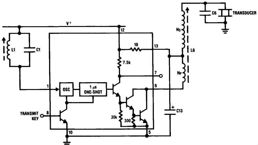
FIGURE 5. Transmitter
