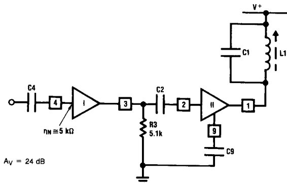
FIGURE 9. Receiver Section
